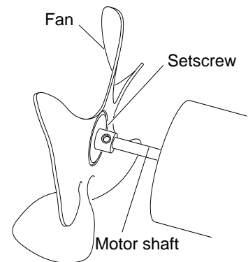
Figure 8 - Fan, Motor Shaft, and Setscrew Location
