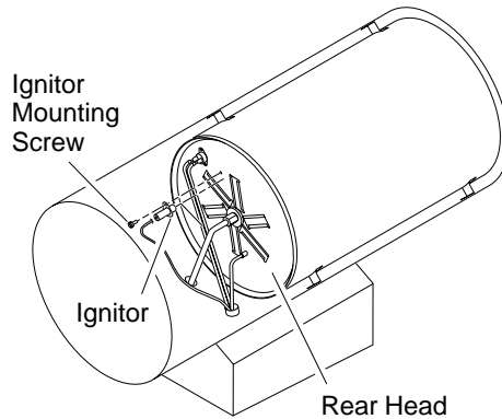
Figure 11 - Removing Ignitor Mounting Screw and Ignitor
