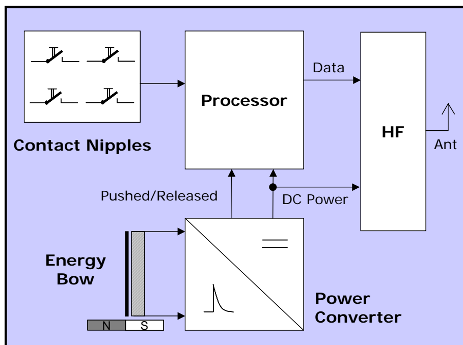
Figure 9: Block diagram of PTM 200C
