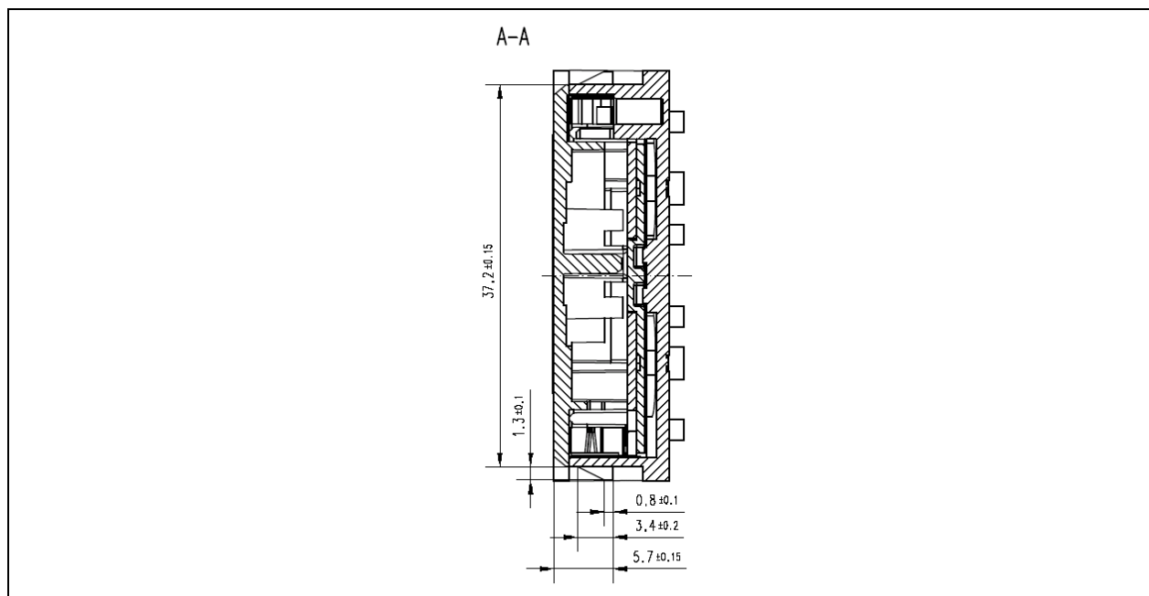
Figure 4: PTM 200C without antenna, cut A
