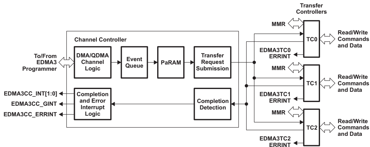
Figure 1. EDMA3 Block Diagram
