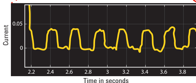
Figure 1. Dynamic current measurement
