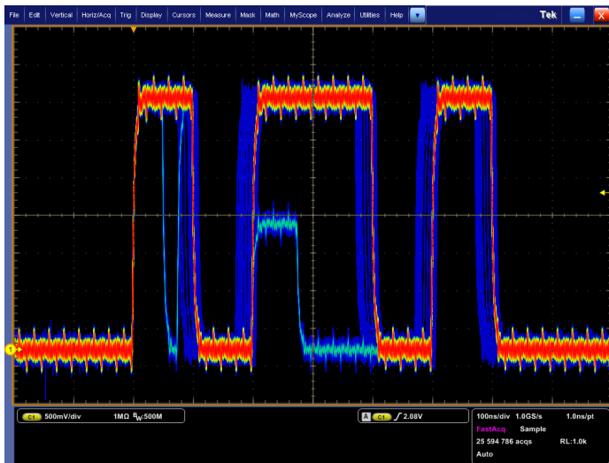
Discover – Fast waveform capture rate - over 250,000 wfm/s - maximizes the probability of capturing elusive glitches and other infrequent events.
