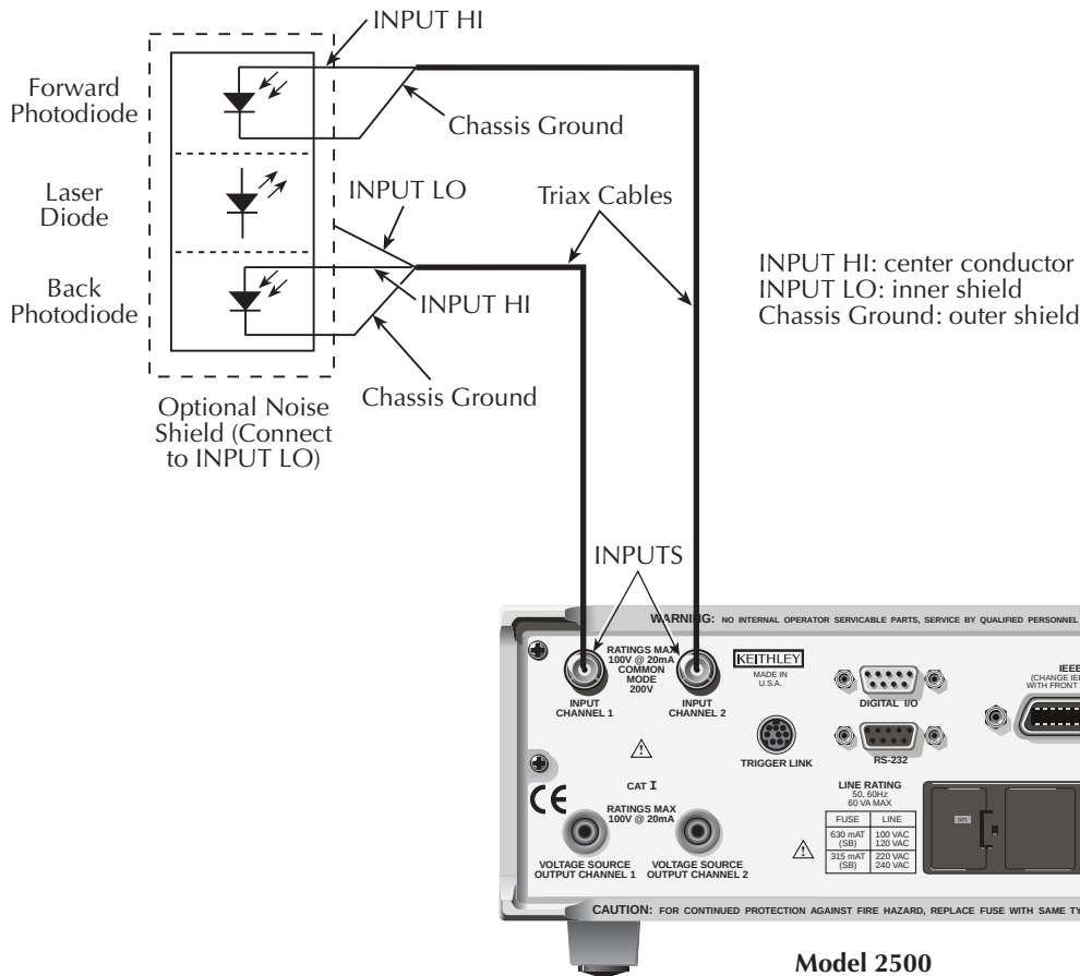
Figure 2-5 Test connections using ground connect mode
