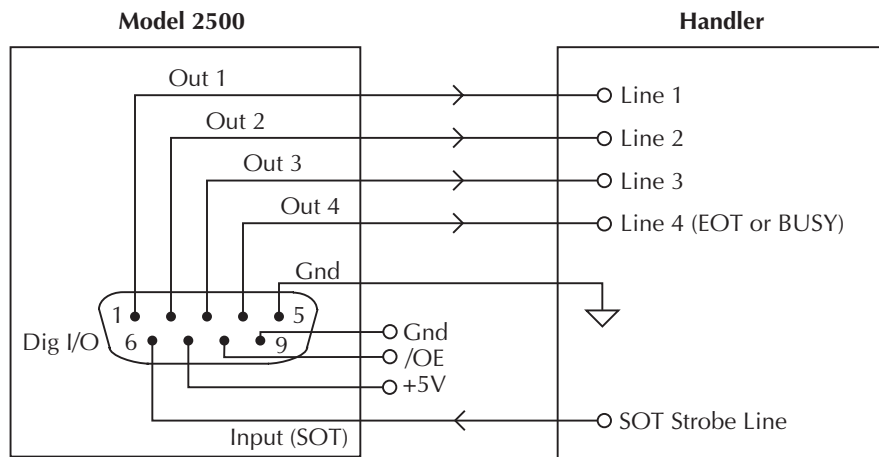
Figure 11-6 Handler interface connections
