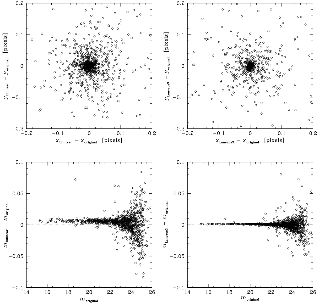
Figure 8: Effects of the resampling on position ( top ) and flux ( bottom ) measurements. Left: bilinear interpolation; right: Lanczos3 interpolation. In both cases, a simulated deep sky image with 0.7'' seeing, containing stars and white background noise, was rotated by 20 degrees and then rotated back to match the original image. Fluxes were measured in a fixed 2'' aperture. The dispersions seen here reflect the differences between measurements on the original and resampled images. These dispersions are much smaller than what one would observe by comparing the measurements on the resampled images with the theoretical (noise-free) positions or fluxes of the simulation. Note however the significant magnitude offset and flux dispersion in the bilinear case, consequences of the stronger smoothing induced by bilinear interpolation.
