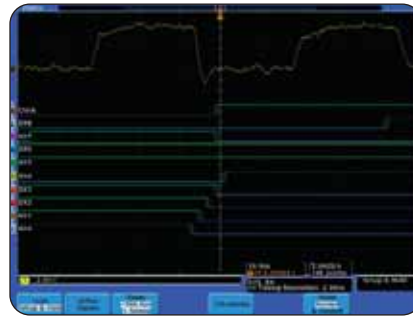
► Multi-channel setup and hold triggering highlighting multiple violations (MSO4000).
