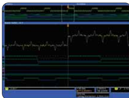
► Wave Inspector® controls provide unprecedented efficiency in viewing, navigating and analyzing waveform data.
