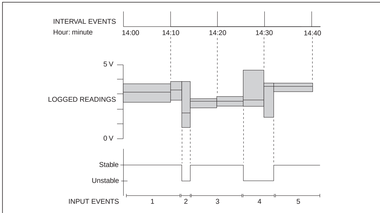
Figure 2. Interval Events and Input Events
