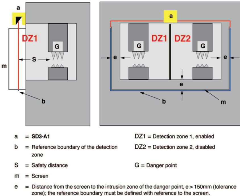
Fig. 5.6-1: Safeguarding of danger point based on hand and arm protection with monitoring of a reference boundary
