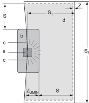
Machine (view from above)
