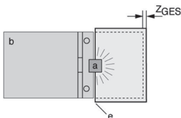
SD3-A1 recessed into the front of a vehicle
