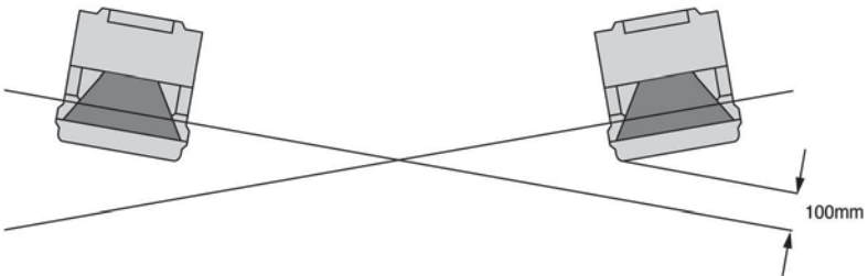
Fig. 5.2-3: Installation without height offset (crossed alignment)
