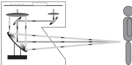
Fig. 2.1-2: Functional principle of the SD3-A1
