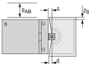
SD3-A1 mounted on the front of a vehicle
