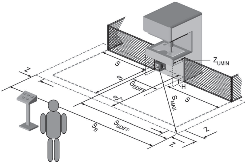
Fig. 5.4-6: The undercut
