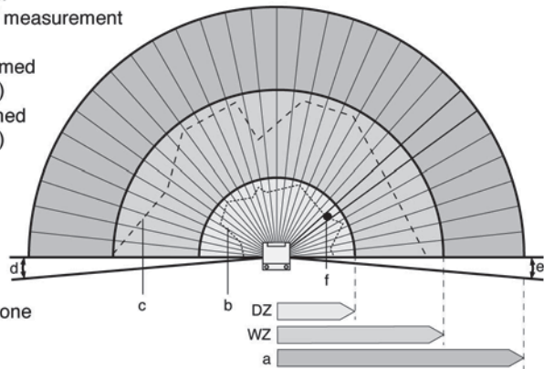
Fig. 2.1-1: The 190° angle range of the SD3-A1 is divided into 0.36° angle segments.
