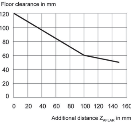
Fig. 5.7-3: Diagram for calculating the addition to compensate for inadequate AGV floor clearance
