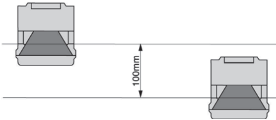
Fig. 5.2-2: Installation with height offset (parallel alignment)
