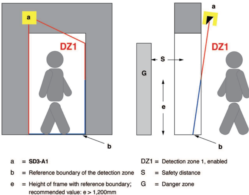
Fig. 5.5-1: Access protection by passage monitoring with system check of a reference boundary
