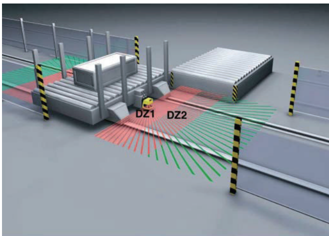
Fig. 4.5-1: Safeguarding a transporter trolley
