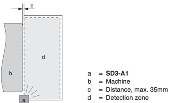
Fig. 5.4-3: Lateral external scanner mounting without an undercut
