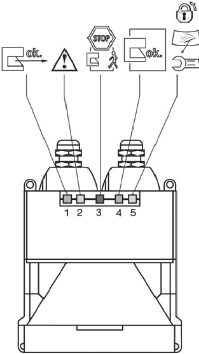
Fig. 10.3-1: The SD3-A1 status indicator
