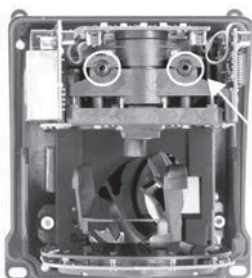
Rubber sleeves
