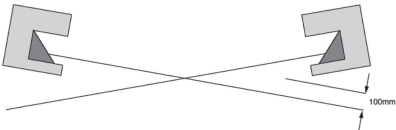
Fig. 5.2-4: Opposing installation without height offset (crossed alignment)
