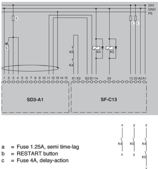
Fig. 8.2-1: Wiring the SD3-A1 with manual restart interlock and relay monitoring, and without zone pair changeover
