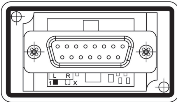
Fig. 10.5-1: SD3-A1 ConfigPlug with switch setting "1"
