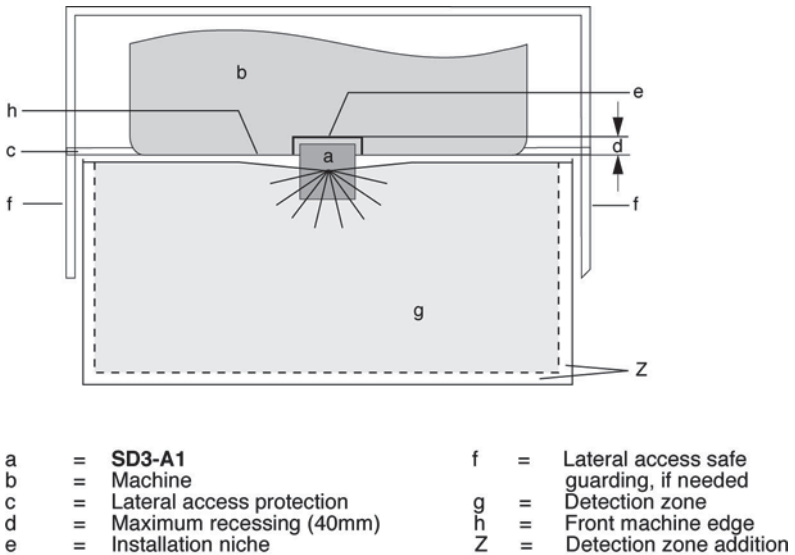
Fig. 5.4-2: Recessed installation within the machine contour
