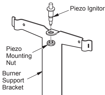
Figure 1 - Installing Piezo Ignitor
