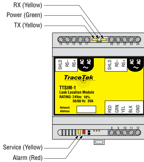
Figure 9. TTSIM-1 LED Locations
