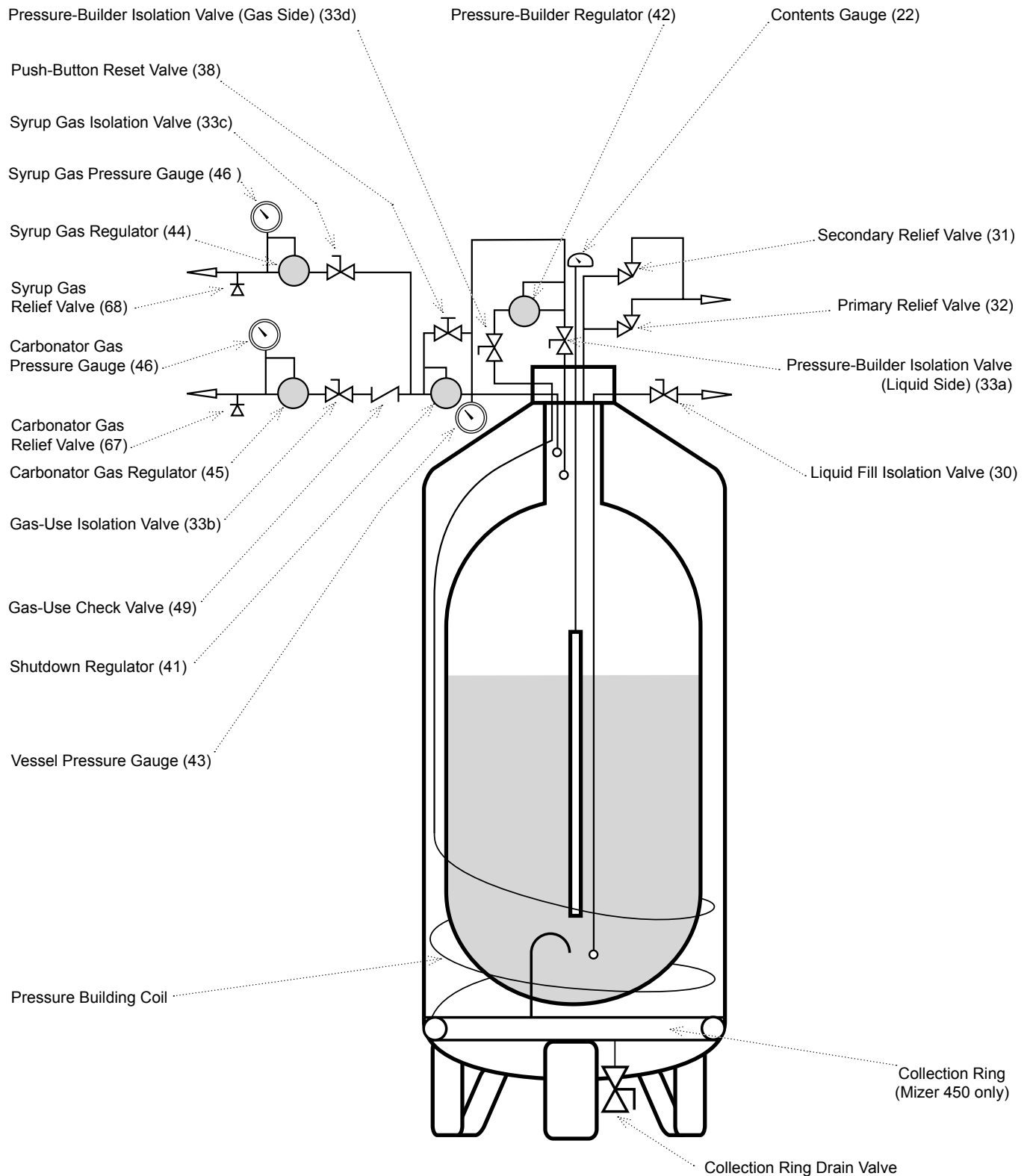
McDonald's Mizer 450 & 750 CO 2 System
