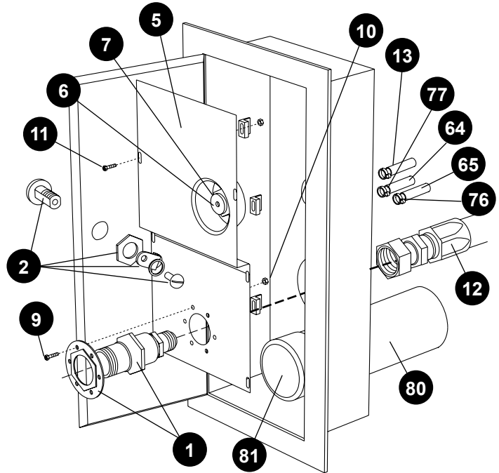
Flush Mount Fill Panel (With Fittings) (P/N 9722859)
