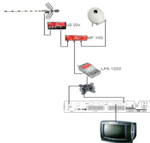
Example 3 - Combined with terrestrial
