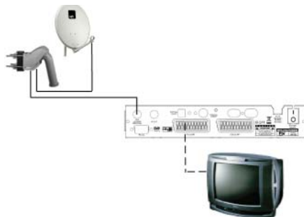
Example 4 - Motorized system
