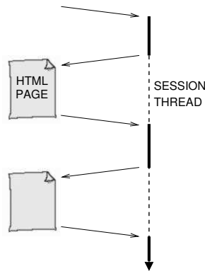
Figure 1: Client-server sessions in Web services. On the left is the client's browser, on the right is a session thread running on the server. The thread is initiated by a client request and controls the sequence of interactions.
