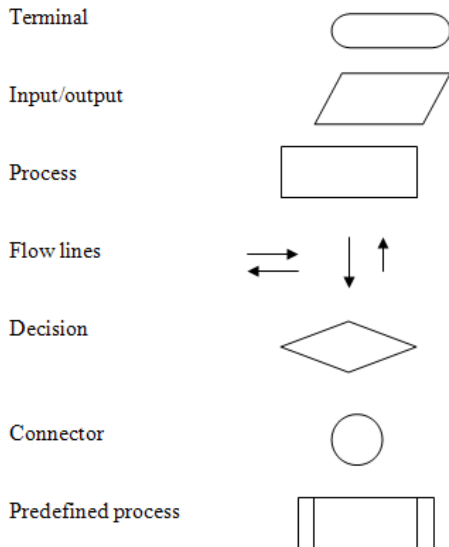
Figure 2.5: Flowchart symbols
