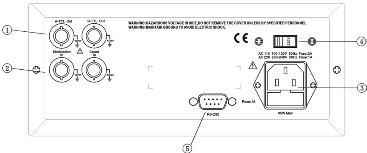
Rear Panel
