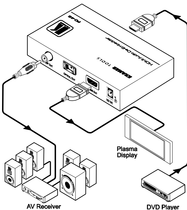
Figure 2: Connecting the FC-46 HDMI Audio De-Embedder
