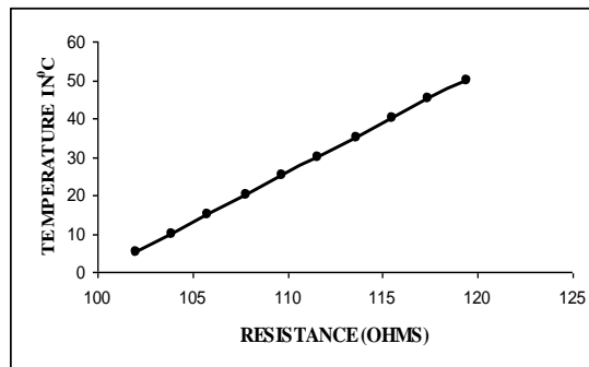
Fig 7 Temperature Measurement
