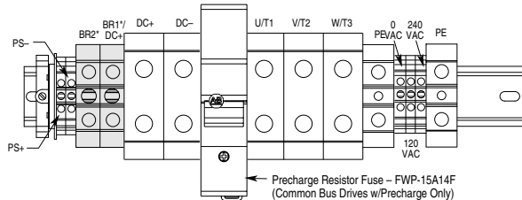
Frame 5 - Common Bus
