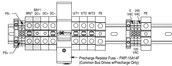
Frame 5 - 100 HP, 480V Normal Duty Drive
