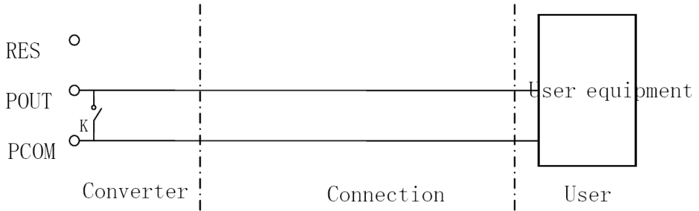
Fig. 8: (a) Digital connect voltage mode
