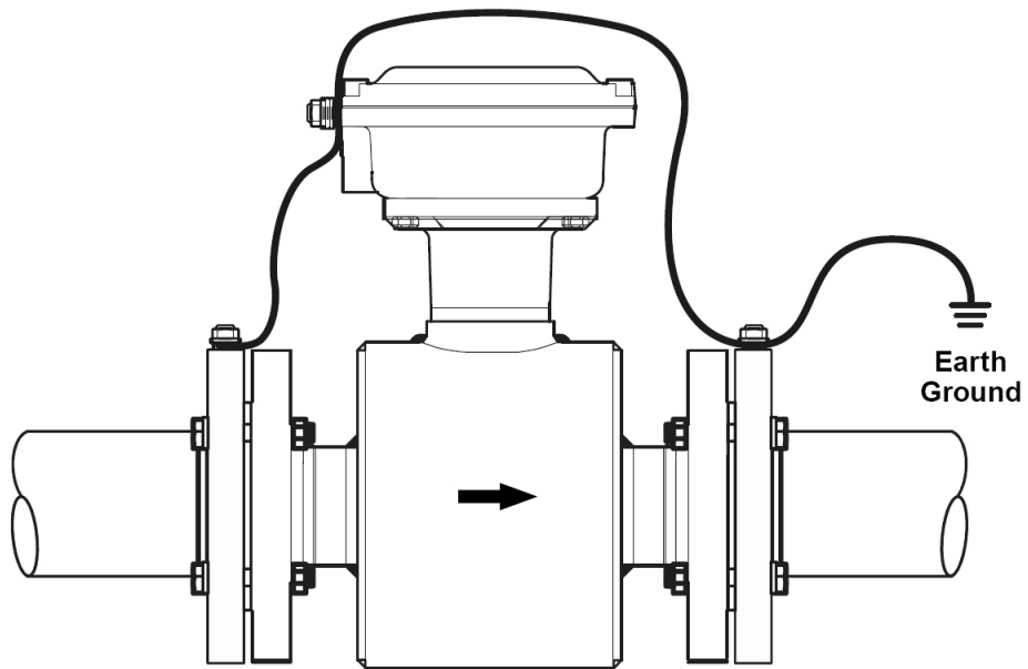
Fig. 15: No Grounding Options or Grounding Electrode in Lined Pipe
