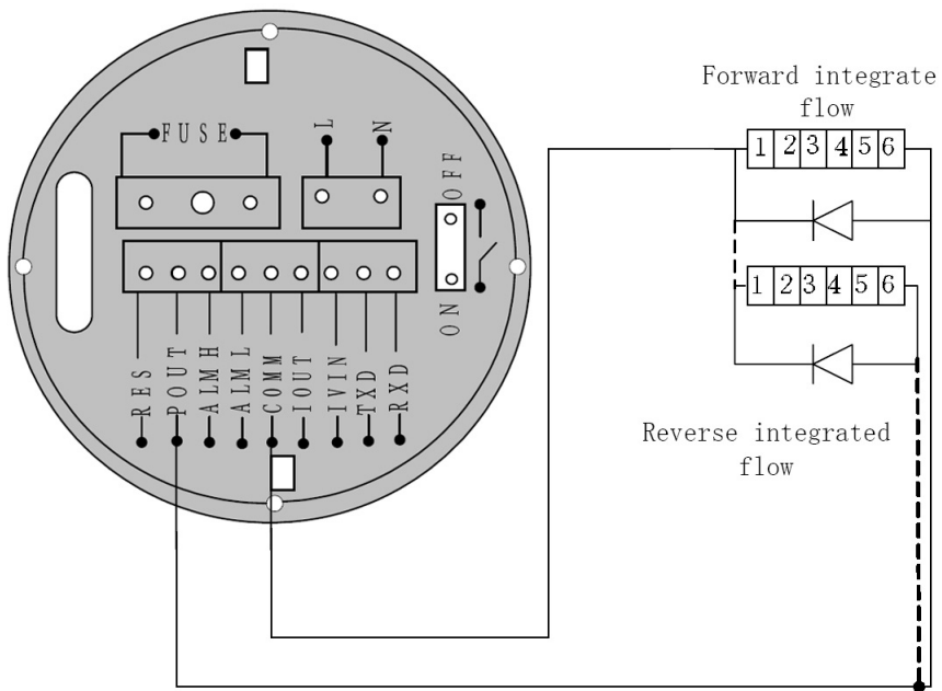
Fig. 7: (c) Connection of Electronic Counter
