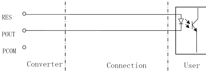
Fig. 8: (b) Digital current connect mode
