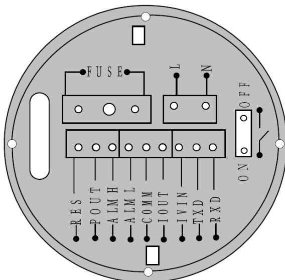
Fig. 6: Labels of connector in Model
