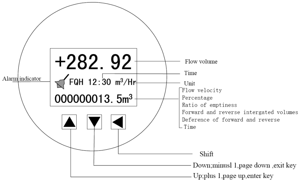
Fig. 5: Define Keys and LCD screen display
