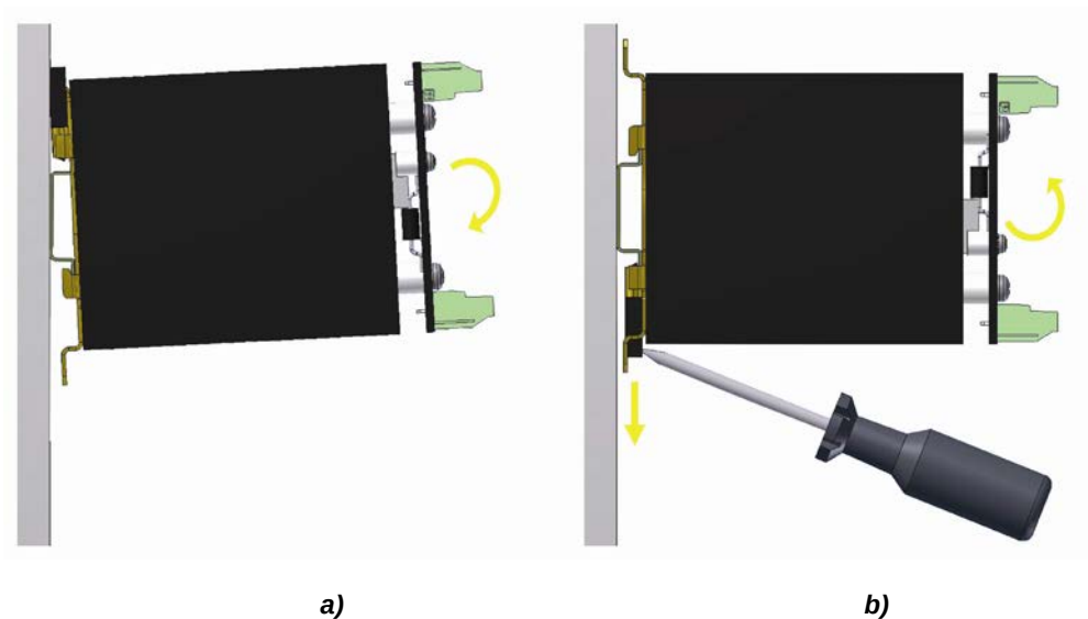
Figure 23 – Assembly (a) and Disassembly (b) of the ITF-DR
