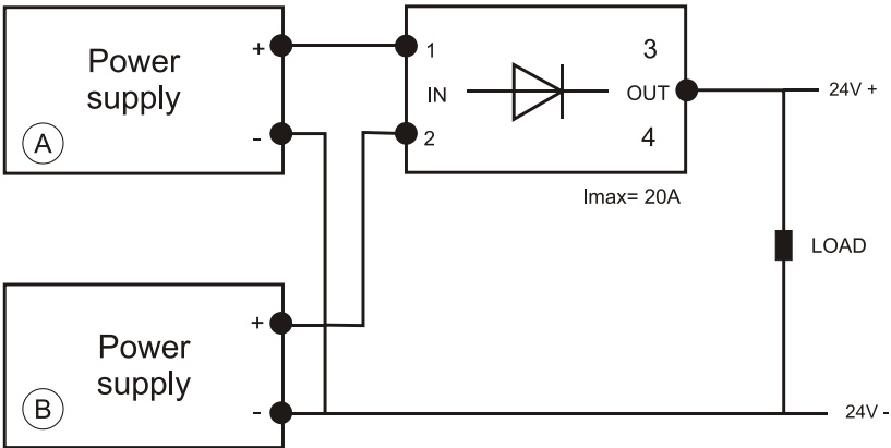
Figure 24 – ITF-DR Interconnection Diagram
