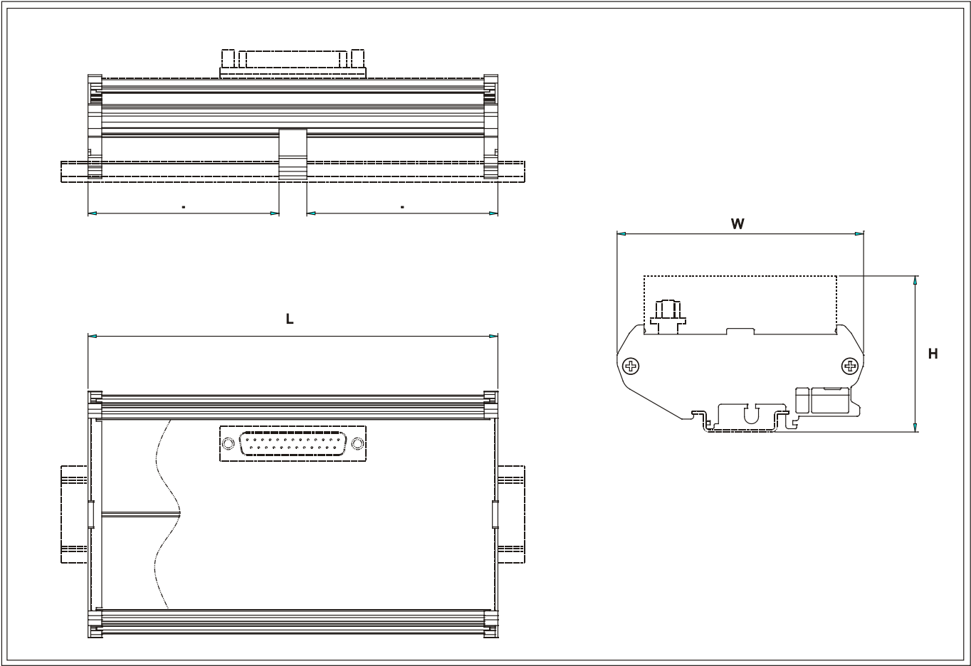
Figure 40 – Dimensional Drawings
