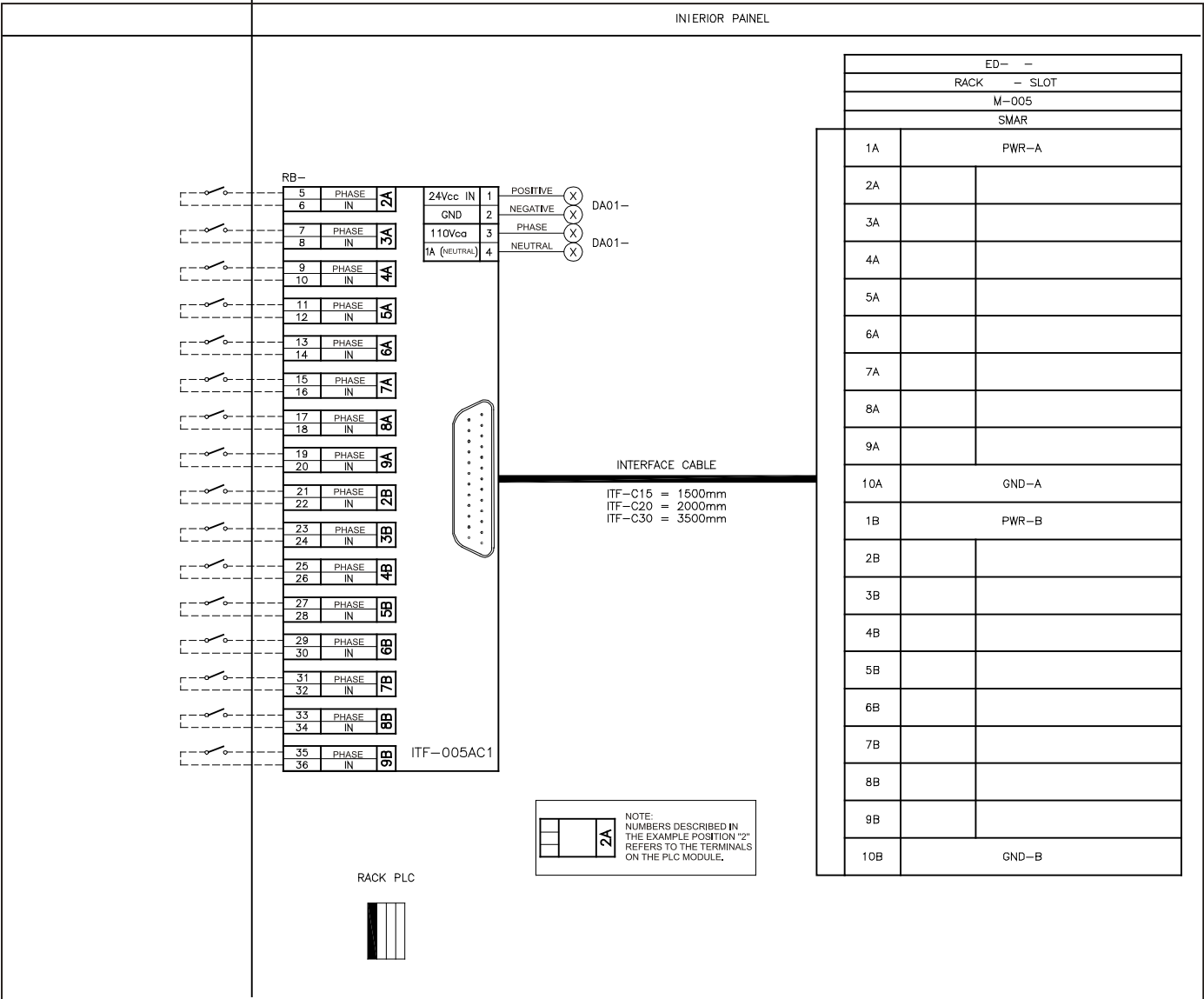
Figure 2 – ITF-005AC1 Interconnection Diagram
