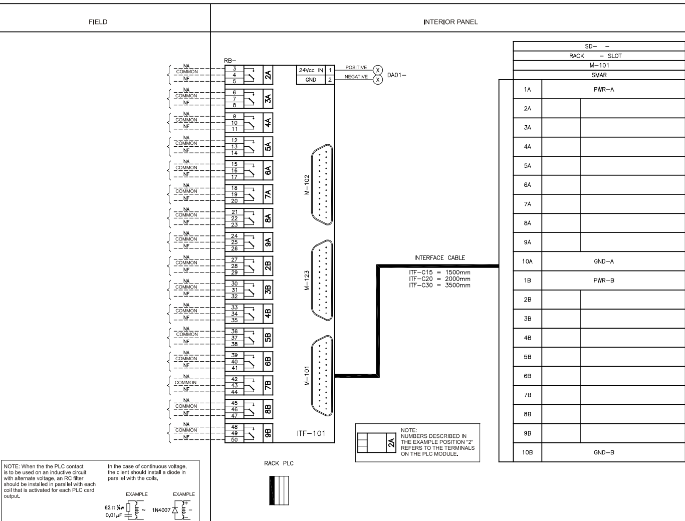
Figure 8 – ITF-101 Interconnection Diagram
