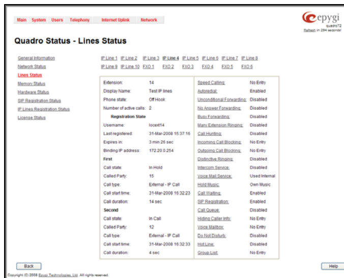
Fig. II-15: Lines Status - Lines Status page upon established call
