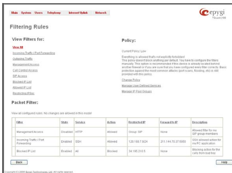
Fig. II-177: Filtering Rules page
