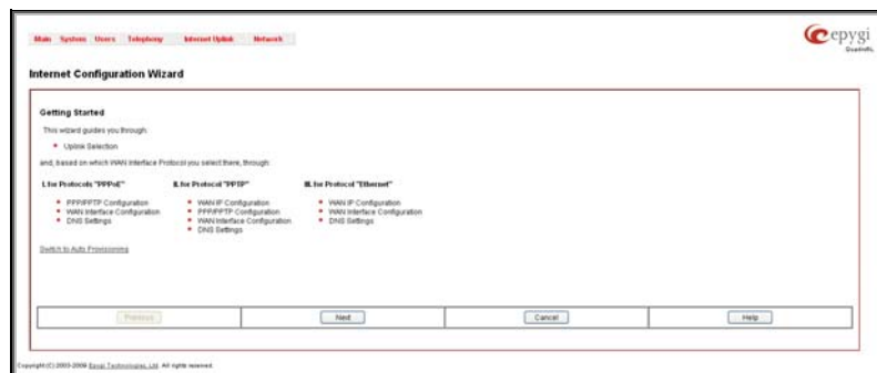
Fig. II-7: Internet Configuration Wizard - Start page
