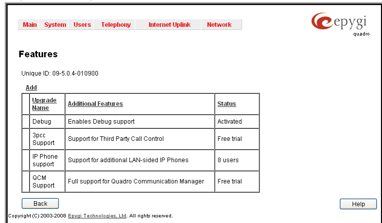
Fig. II-56: Features page
