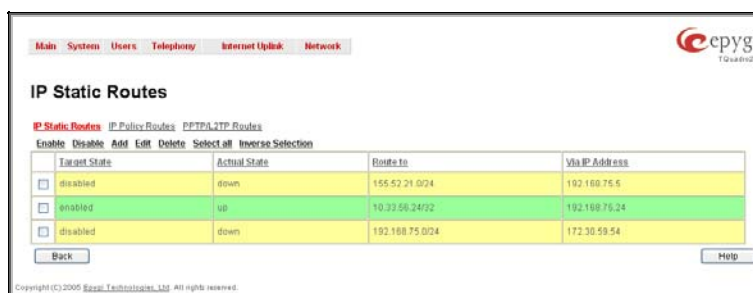
Fig. II-25: IP Static Routing table
