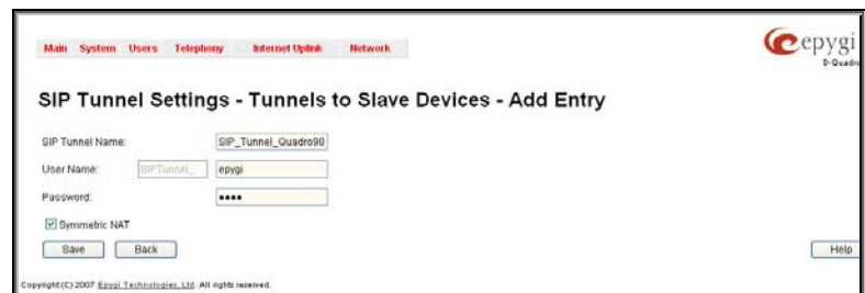
Fig. II-133: SIP Tunnel Settings – Tunnels to Slave Devices – Add Entry page
