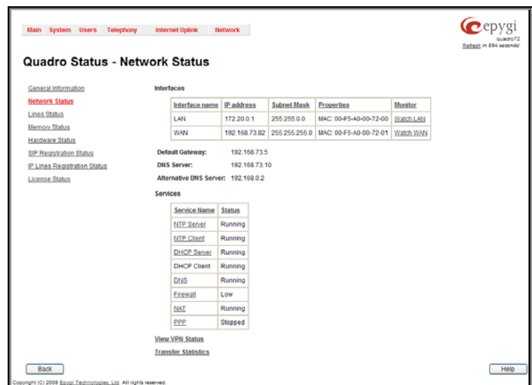
Fig. II-12: Quadro Status Network Status page
