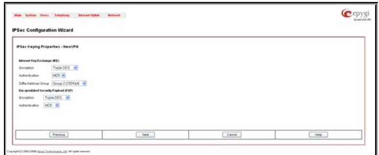
Fig. II-165: IPsec Connection Wizard -IPsec Connection Properties
