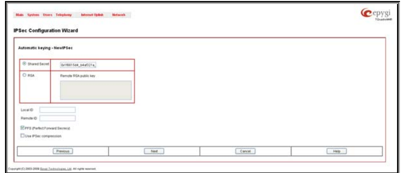
Fig. II-166: IPSec Connection Wizard - Automatic Keying Settings page
