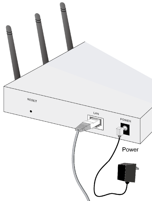
Figure 4: Installation Diagram
