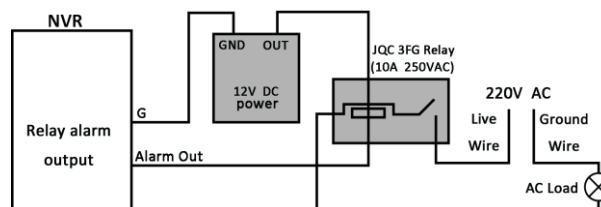
AC Load Connection Diagram
