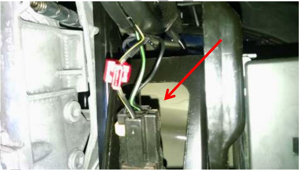
Figure 4 (Brake Sensor)
