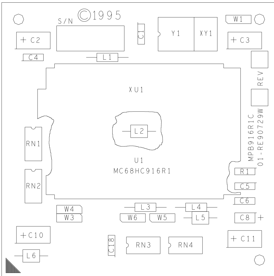
Figure 2-1. M68MPB916R1 (C version) Parts Location Diagram (top view)
