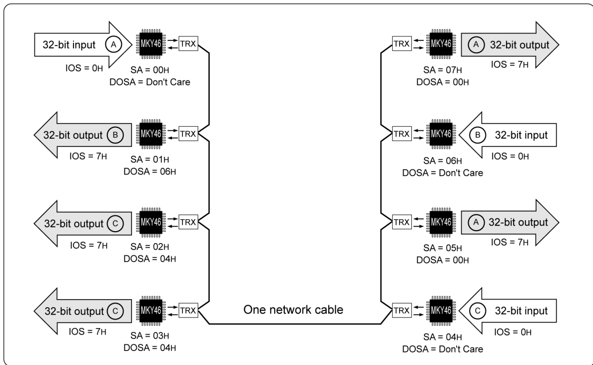
Fig. 4.14 Concept of System Where Multiple I/O Signals Can Be Connected with One Network Cable
