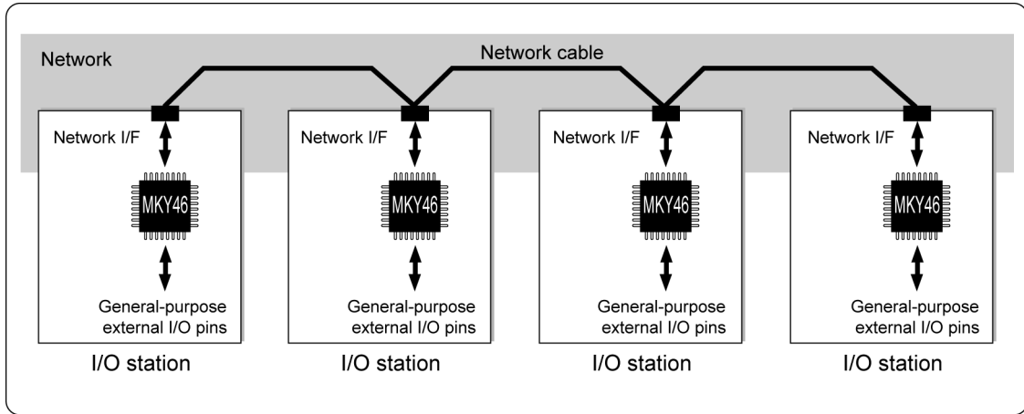
Fig. 4.13 CUnet Configured Only by I/O Stations
