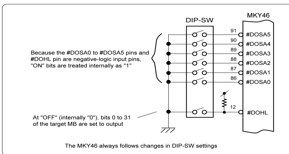
Fig. 4.6 Setting Example of #DOSA0 to #DOSA5 Pins and #DOHL Pin
