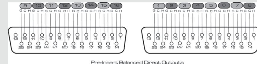
DB25 Pinout
