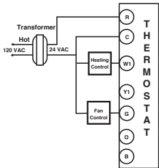
HEAT ONLY 3-WIRE SINGLE TRANSFORMER
