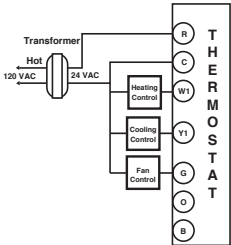
HEAT/COOL 4-WIRE SINGLE TRANSFORMER
