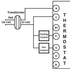
COOL ONLY 3-WIRE SINGLE TRANSFORMER
