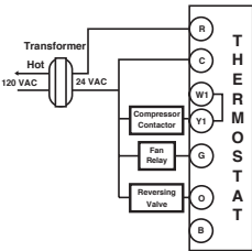
HEAT PUMP WITH COOL ACTIVE REVERSING VALVE
