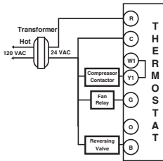
HEAT PUMP WITH HEAT ACTIVE REVERSING VALVE
