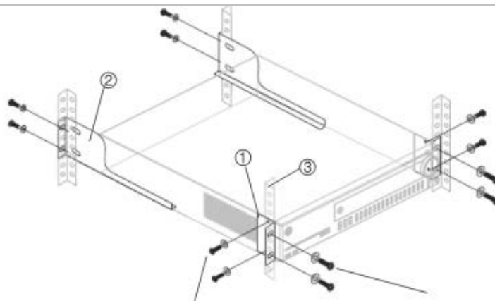
Figure 6: Rack-mount installation
