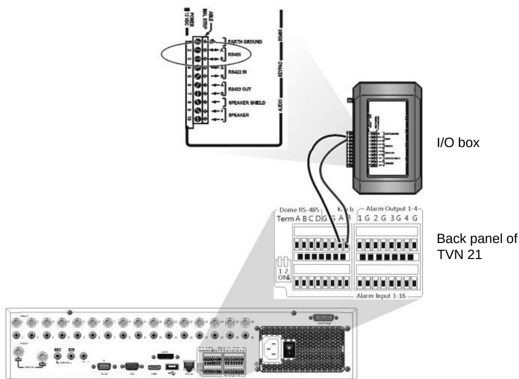
Figure 41: Keypad and NVR connections
