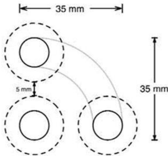
Figure 5. Area required for performing the Two-Finger Pivot Rotate gesture.
