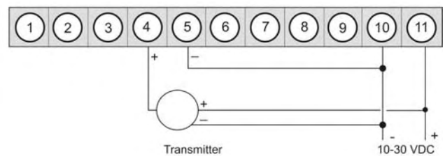
M2 in combination with a 3-wire-sensor 0/4-20 mA
