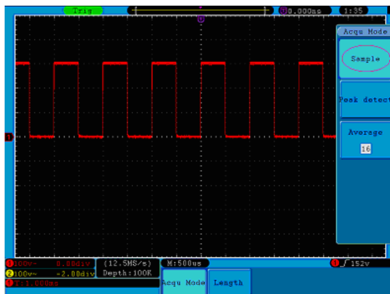
Figure 43. Normal ACQU Mode display, in which no burr can be detected.
