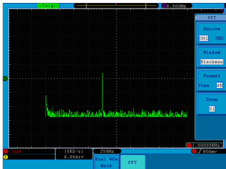
Figure 27. Blackman window.
