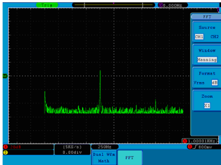
Figure 26. Hanning window.
