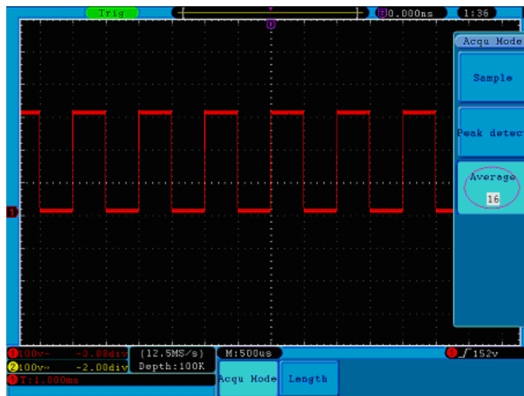
Figure 86. Reduce Noise level by using Average function.
