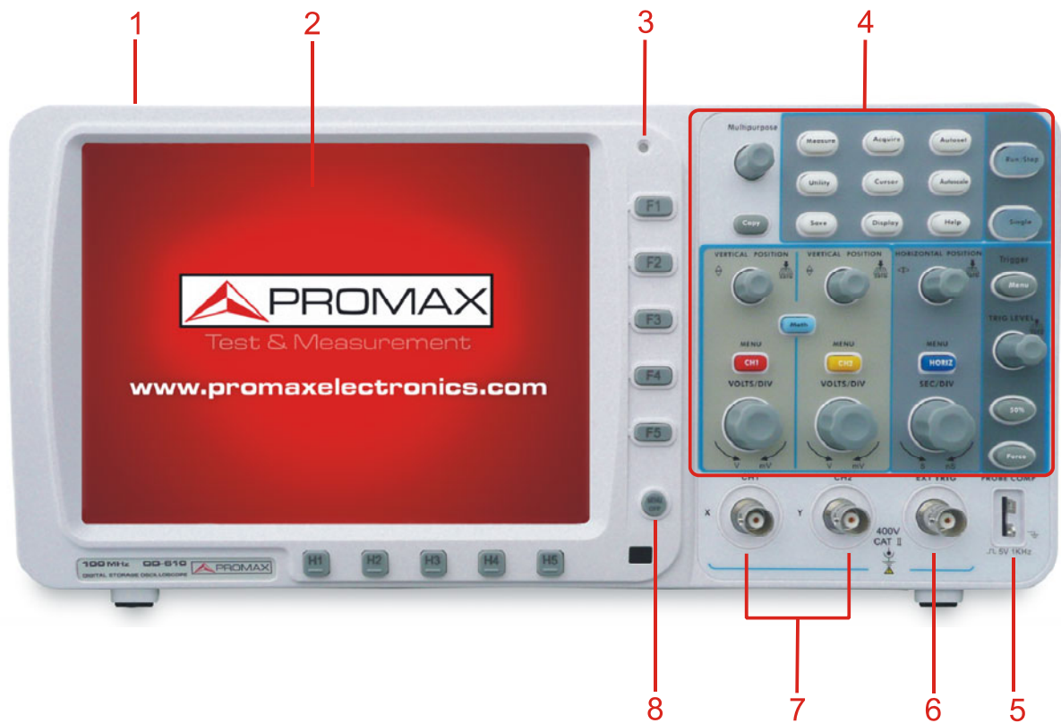
Figure 1. Front Panel.
