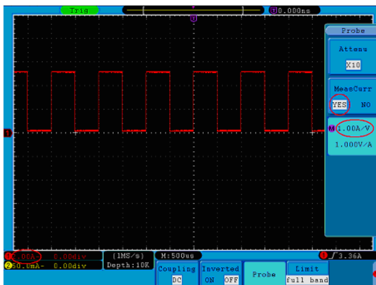
Figure 19. Regulation of the Attenuation Ratio of the Probe.
