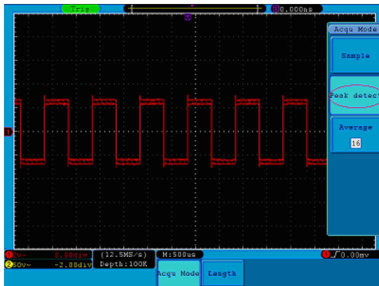
Figure 42. Peak Detect mode, under which the burrs on the falling edge of the square wave, can be detected and the noise is heavy.
