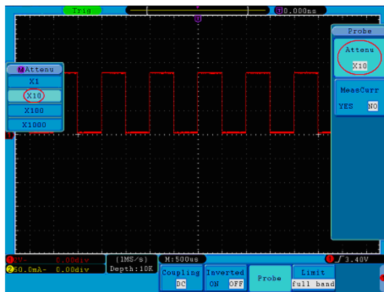
Figure 18. Regulation of the Attenuation Ratio of the Probe.
