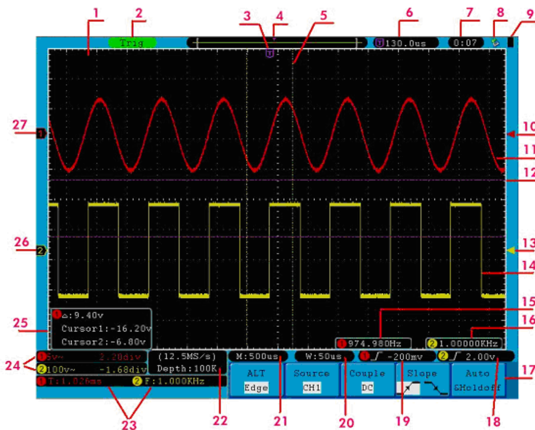
Figure 6. Illustrative Drawing of Display Interfaces.
