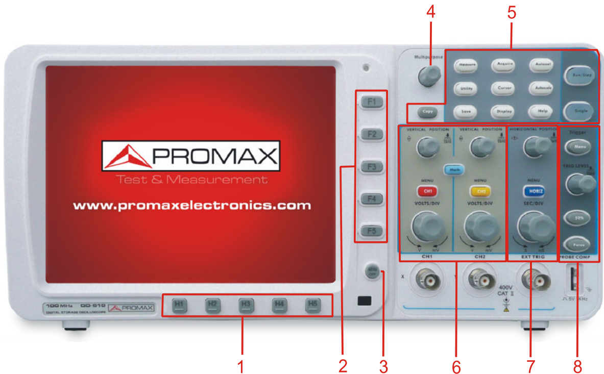
Figure 5. Keys Overview
