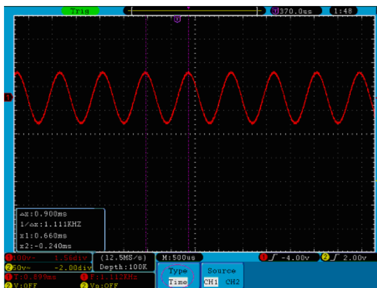
Figure 70. Waveform of Cursor Measurement.
