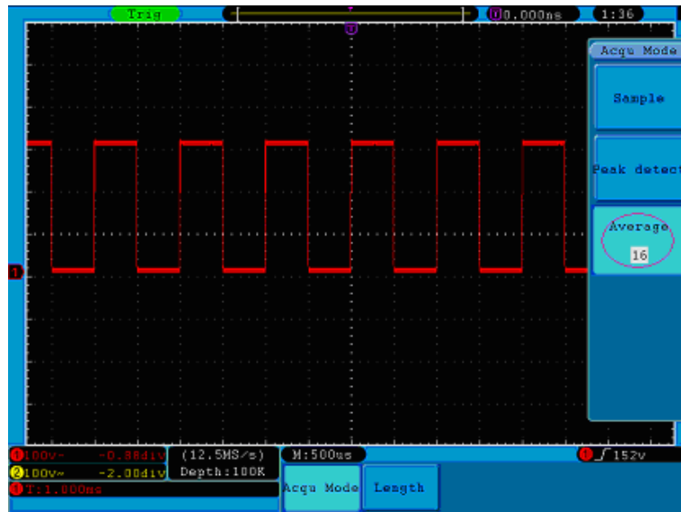
Figure 44. The displayed waveform after the noise is removed under the Average Mode, in which the average number of 16 is set.
