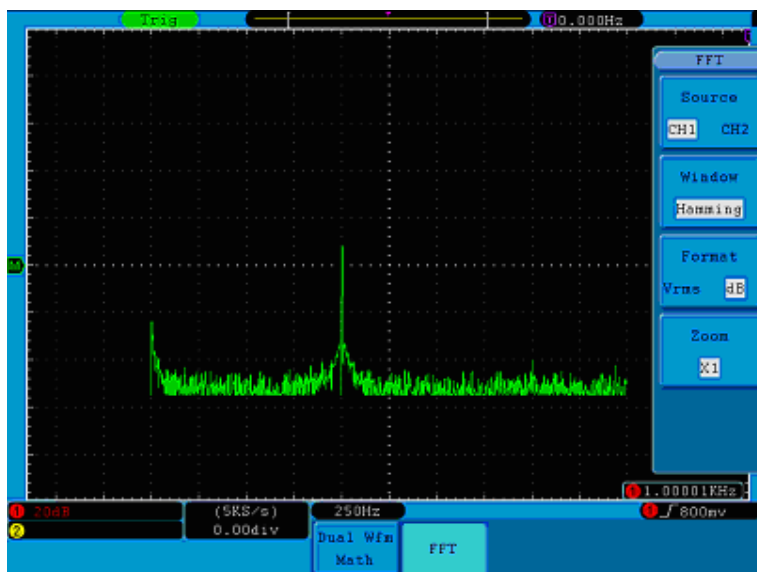
Figure 25. Hamming window.
