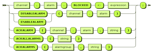
Syntaxgraph 17: alarm_statements
