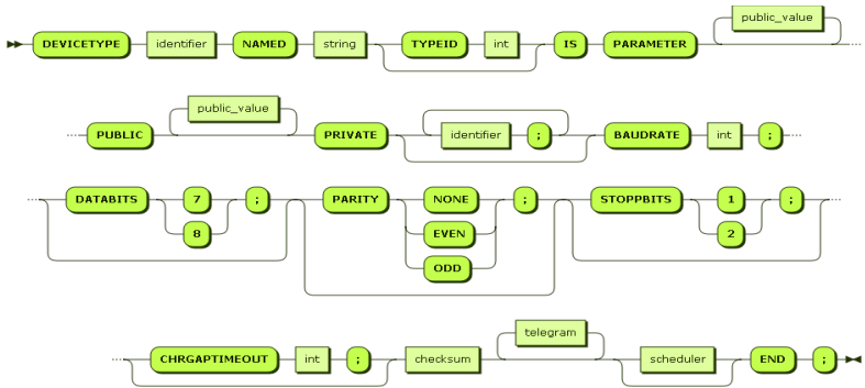
Syntaxgraph 23: devicetype
