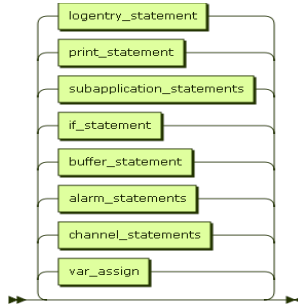
Syntaxgraph 4: statements
