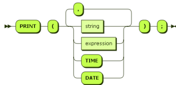
Syntaxgraph 7: print_statement
