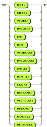
Syntaxgraph 36: telegram_datatype
