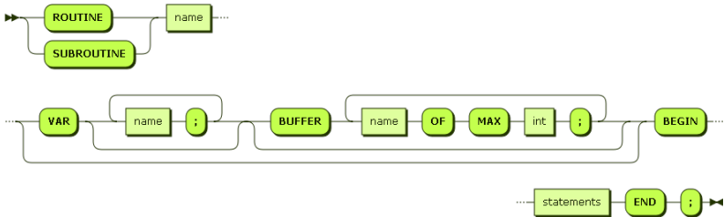
Syntaxgraph 3: routine
