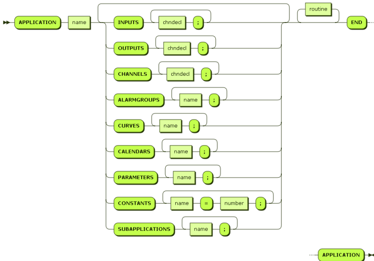
Syntaxgraph 1: application
