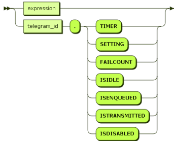
Syntaxgraph 35: expression_SchedulerMode_
