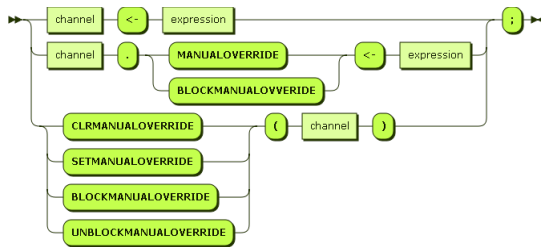
Syntaxgraph 15: channel_statements
