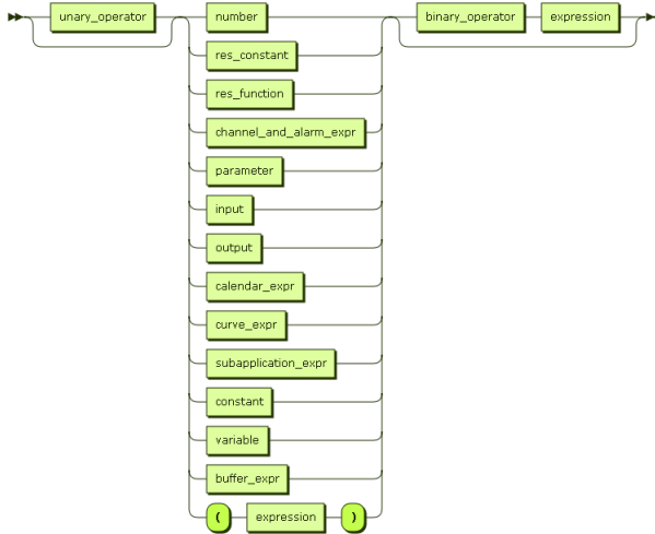
Syntaxgraph 9: expression
