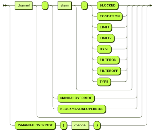
Syntaxgraph 16: channel_and_alarm_expressions
