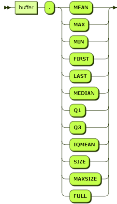
Syntaxgraph 22: buffer_expression
