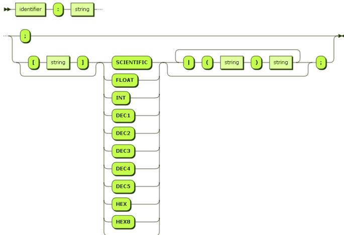
Syntaxgraph 24: public_value
