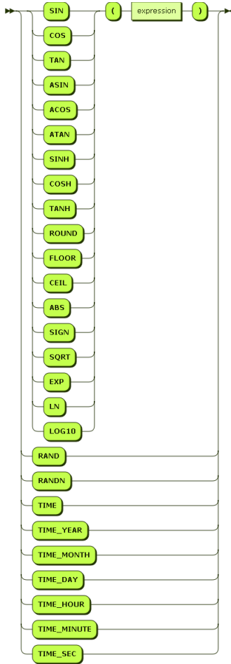
Syntaxgraph 14: reserved_function
