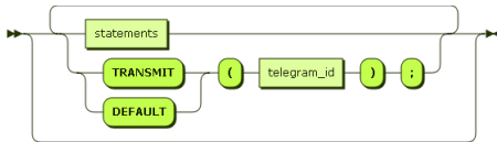
Syntaxgraph 34: statements_SchedulerMode_
