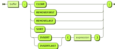
Syntaxgraph 21: buffer_statement
