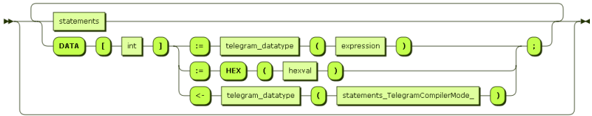
Syntaxgraph 29: statement_TelegramCompilerMode_
