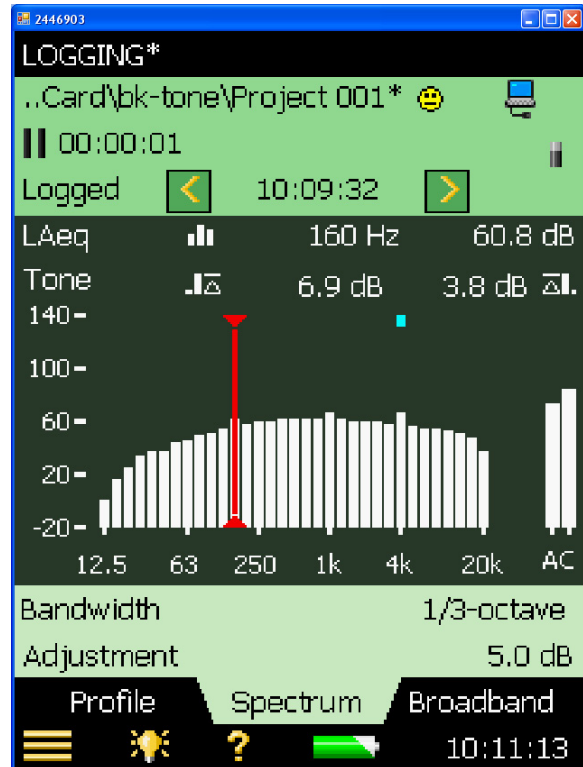
Figure 3 The result display for tone assessment using the simplified, 1/3 octave based method
