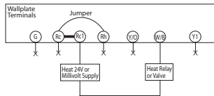
2-Wire Heat Only System
