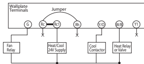
4-Wire Heat/Cool System
