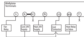
5-Wire Heat/Cool System
