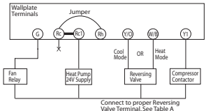
Single-Stage Heat Pump System
