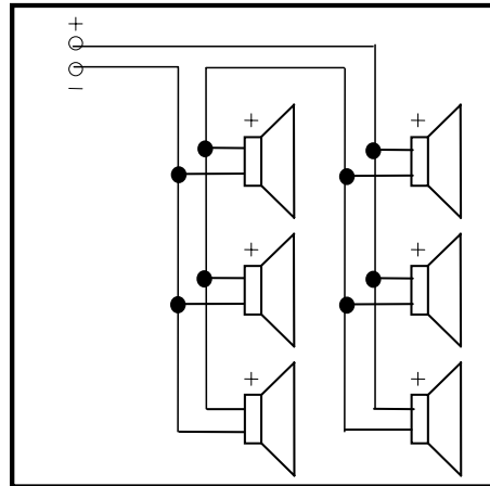
6 Speakers of 16 (8) Ohms Total load of 10.6 (5.3) Ohms
