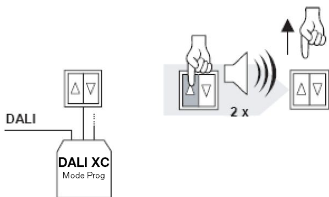
Figure 10: Starting system extension (DALI XC in "Prog" operating mode)
