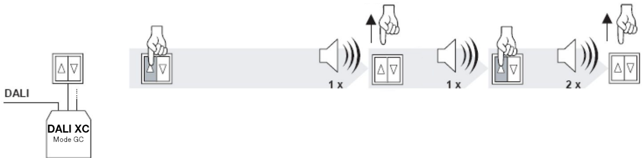
Figure 11: Starting system extension (DALI XC in "GC" operating mode)
