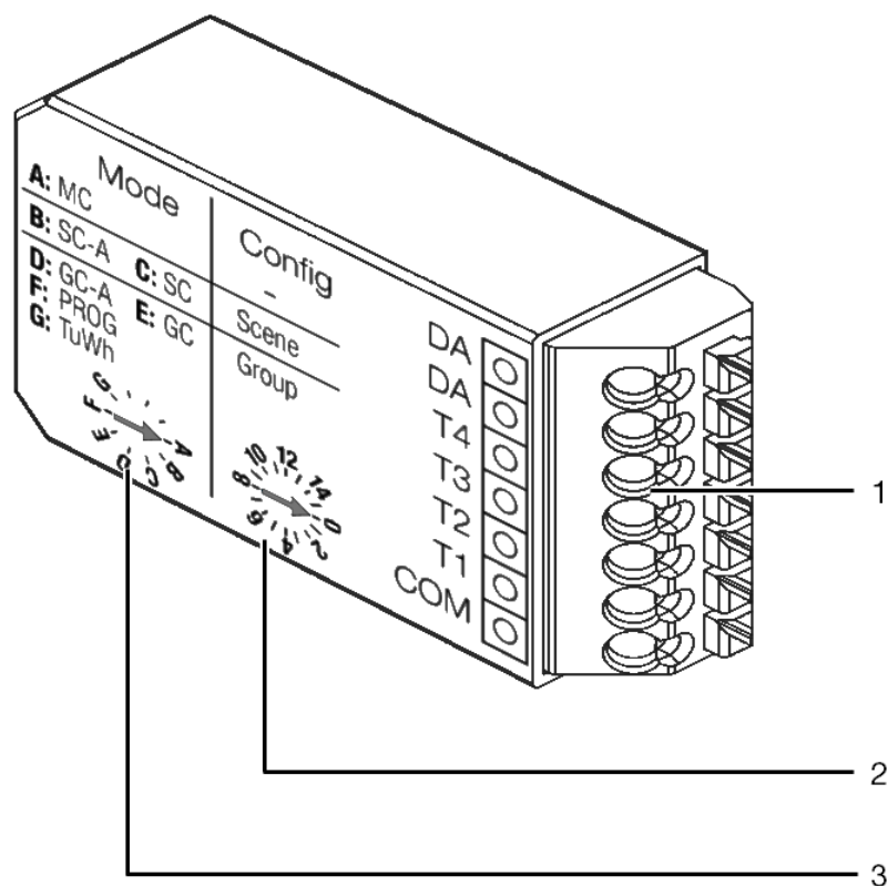
Figure 1: DALI XC input device
