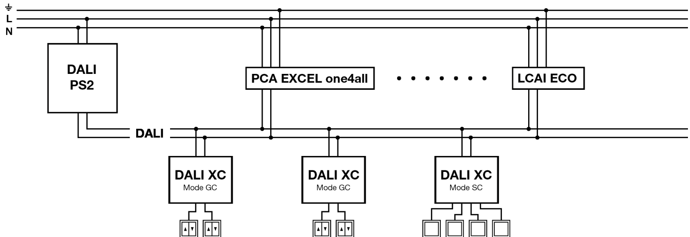
Figure 2: DALI XC in a lighting system as part of the comfortDIM system
