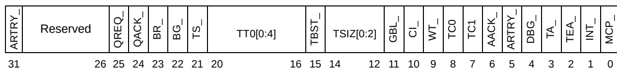
Figure 18-2. Watchpoint #1 Control Trigger Register (WP1_CNTL_TRIG)— Offsets 0xF_F018, 0xF18
