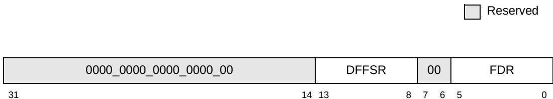
Figure 10-4. I 2 C Frequency Divider Register (I2CFDR)
