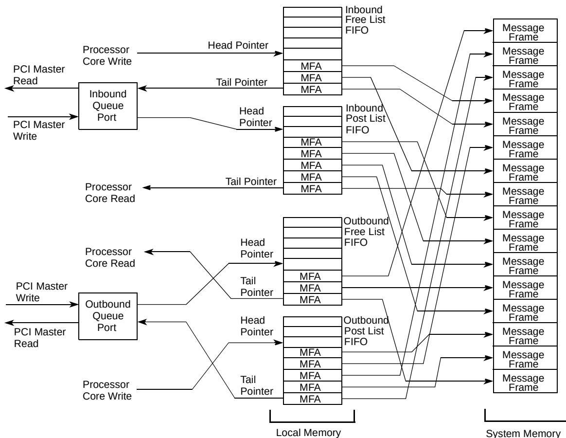
Figure 9-4. I 2 O Message Queue Example
