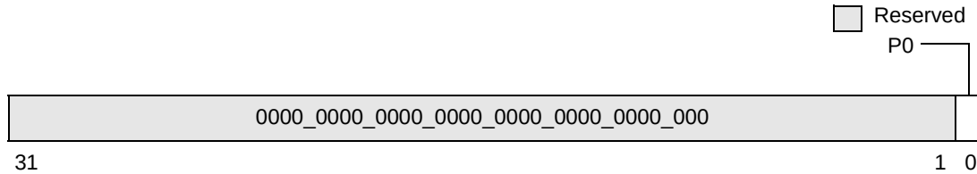
Figure 11-17. Direct and Serial Destination Registers (IDR and SIR)
