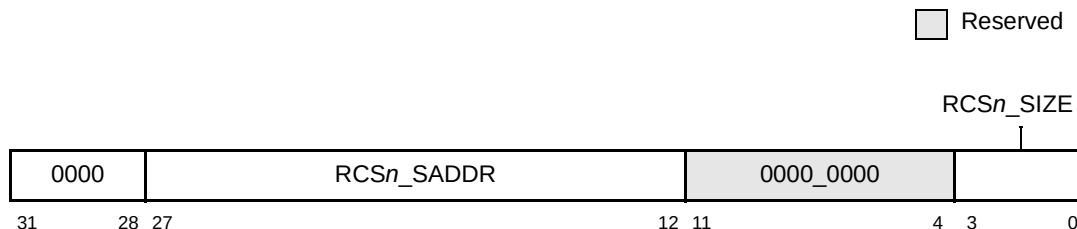
Figure 4-29. ERCCR3 and ERCCR4—0xD8, 0xDC
