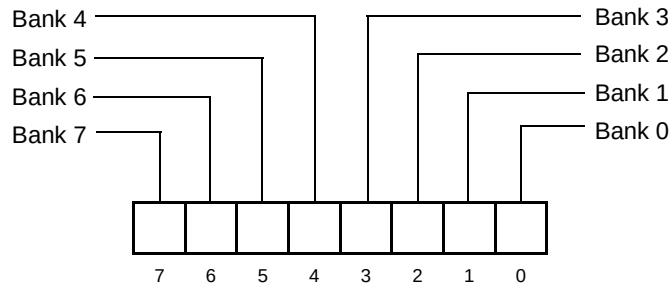
Figure 4-15. Memory Bank Enable Register—0xA0
