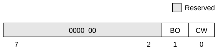
Figure 12-15. Alternate Function Register (UAFR)
