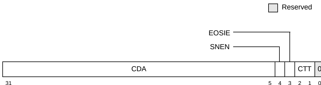
Figure 8-6. Current Descriptor Address Register (CDAR)
