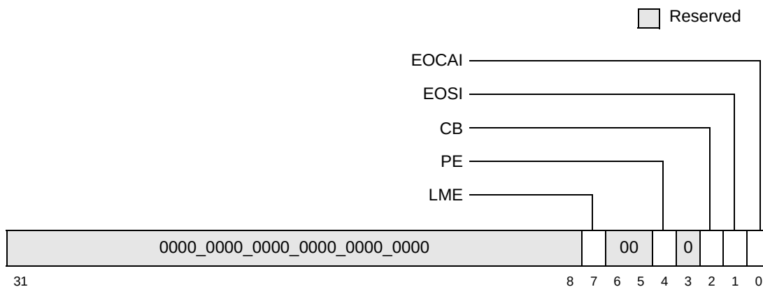
Figure 8-5. DMA Status Register (DSR)
