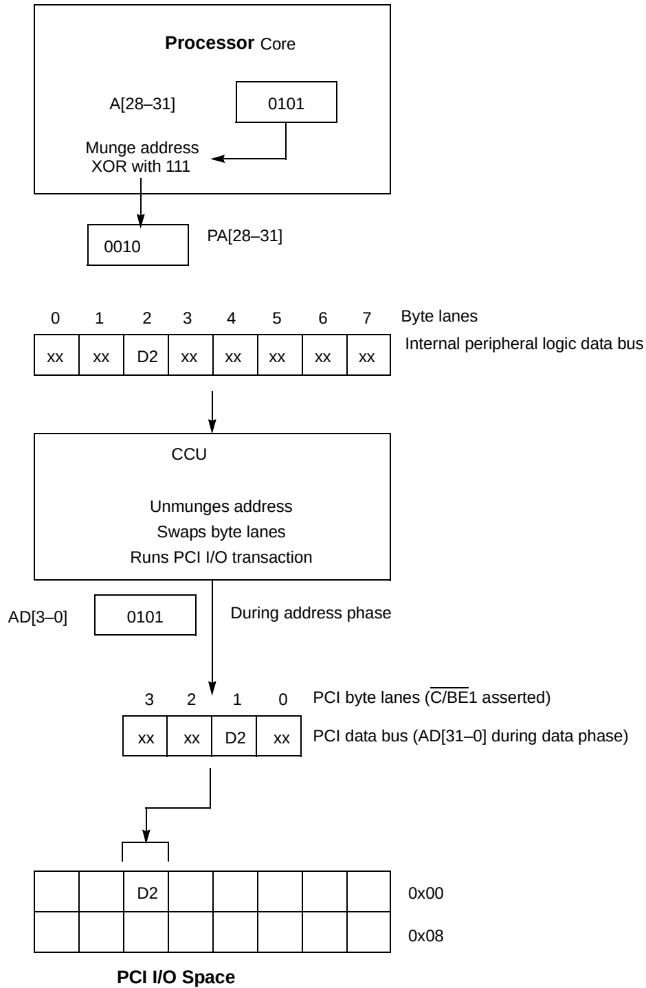
Figure A-9. One-Byte Transfer to PCI I/O Space—Little-Endian Mode
