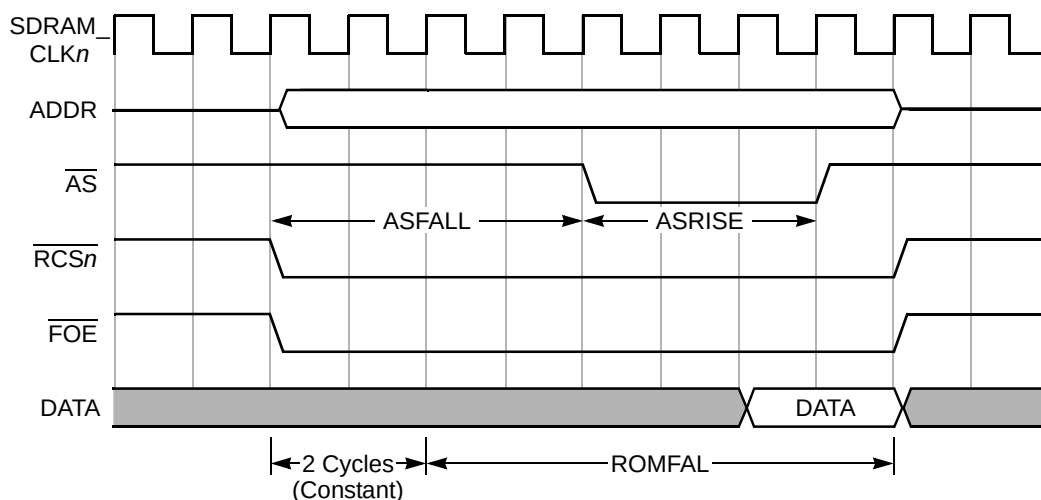
Figure 6-47. Port X Read Access Timing
