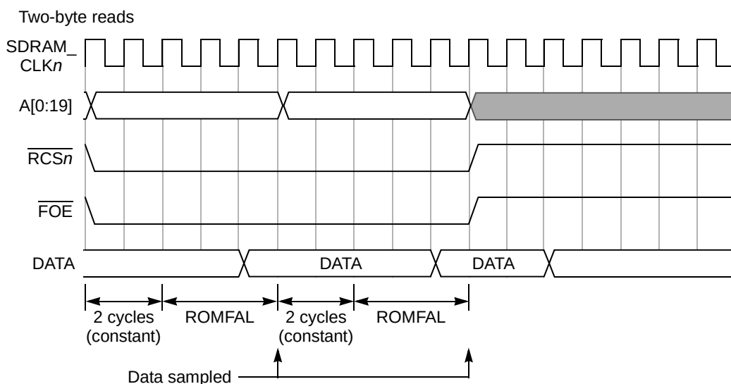
Figure 6-42. 8-Bit ROM/Flash Interface—Two-Byte Read Timing
