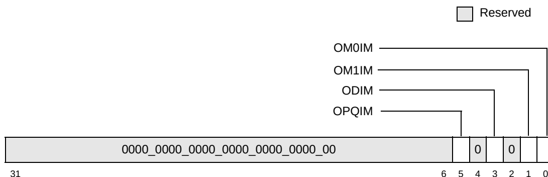
Figure 9-6. Outbound Message Interrupt Mask Register (OMIMR)
