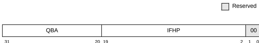
Figure 9-11. Inbound Free_FIFO Head Pointer Register (IFHPR)
