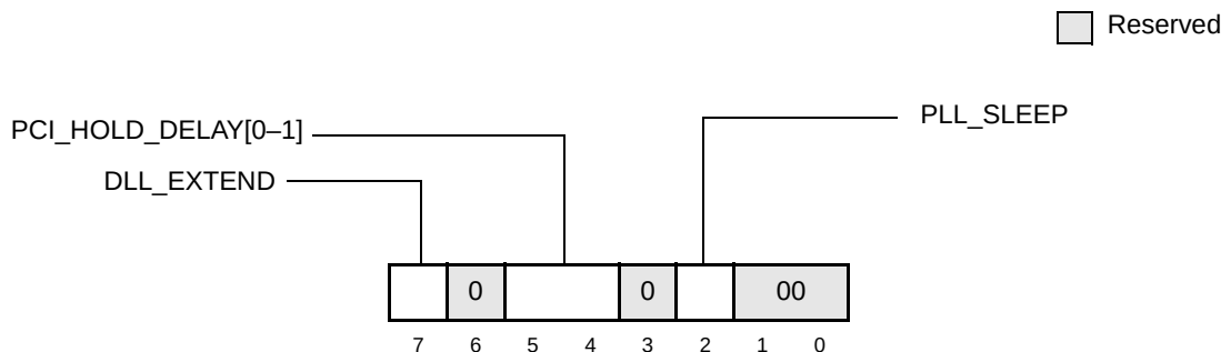
Figure 4-6. Power Management Configuration Register 2 (PMCR2)—0x72
