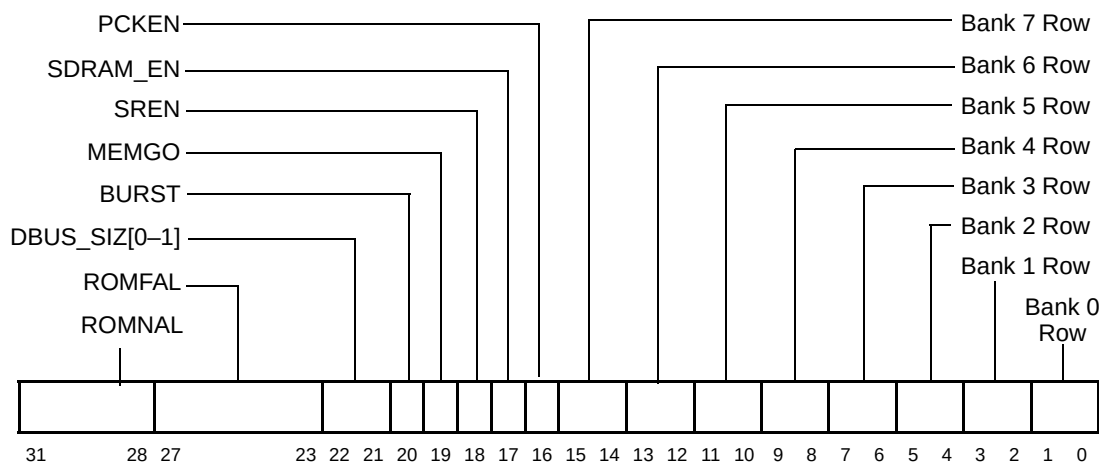
Figure 4-33. Memory Control Configuration Register 1 (MCCR1)—0xF0
