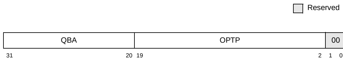
Figure 9-18. Outbound Post_FIFO Tail Pointer Register (OPTPR)
