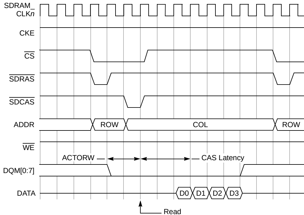
Figure 6-11. SDRAM Four-Beat Burst Read Timing Configuration—64-Bit Mode
