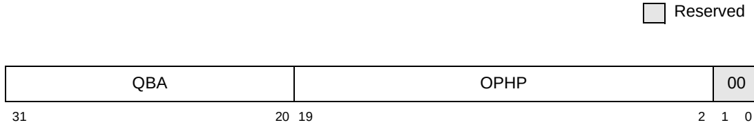
Figure 9-17. Outbound Post_FIFO Head Pointer Register (OPHPR)
