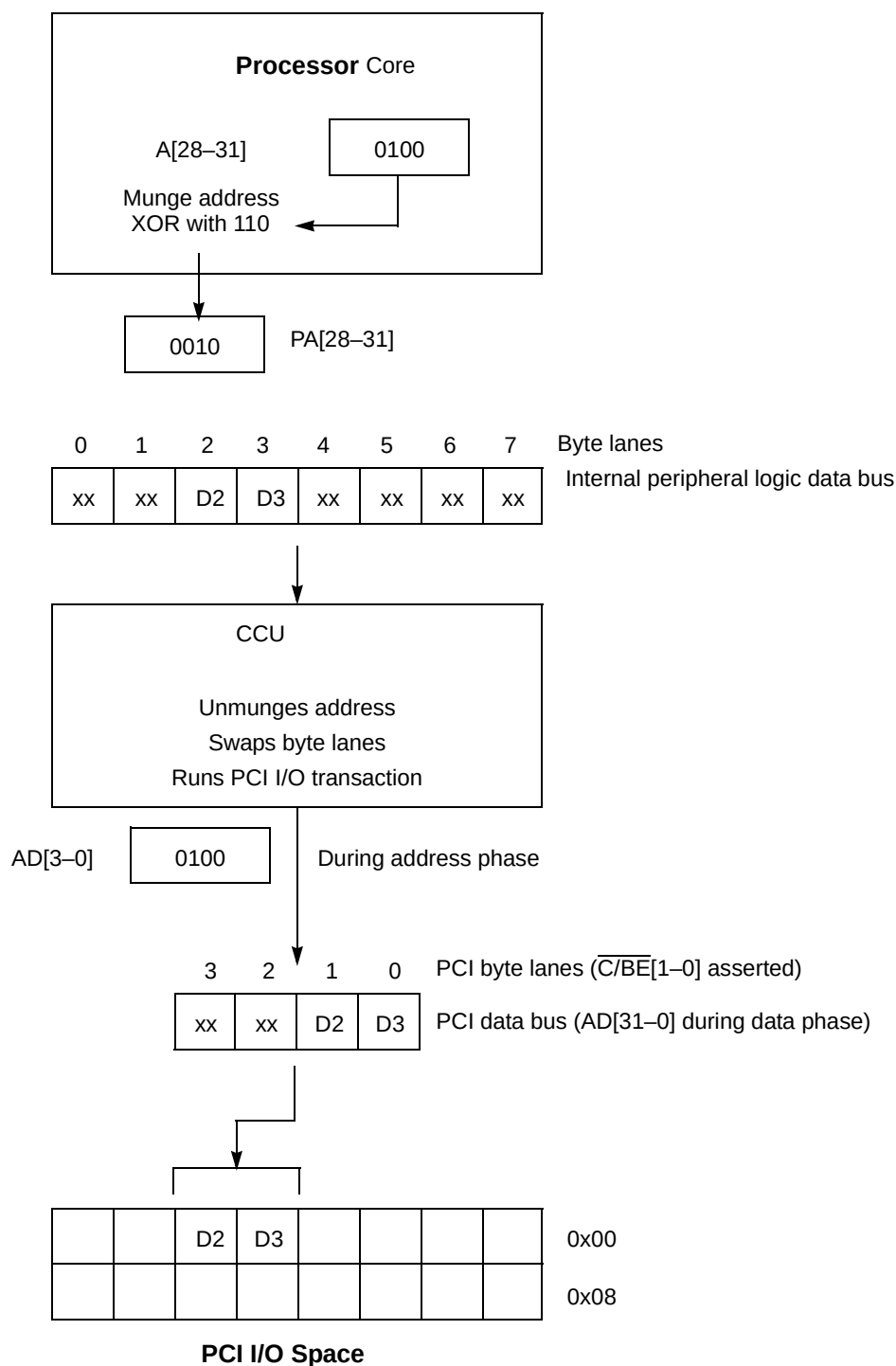
Figure A-10. Two-Byte Transfer to PCI I/O Space—Little-Endian Mode
