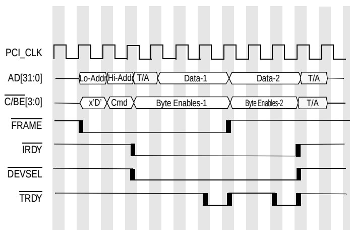
Figure 7-9. DAC Burst Read Example
