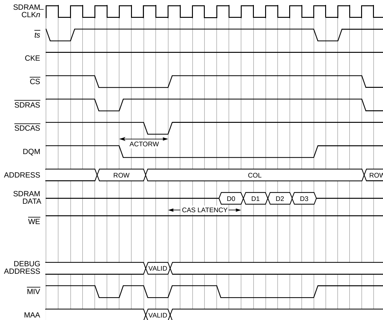
Figure 17-9. SDRAM Debug Address, \overline{\text{MIV}} , and MAA Timings for Burst Read Operation
