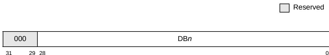
Figure 9-3. Outbound Doorbell Register (ODBR)
