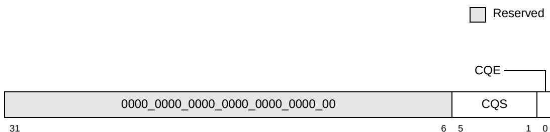
Figure 9-19. Messaging Unit Control Register (MUCR)
