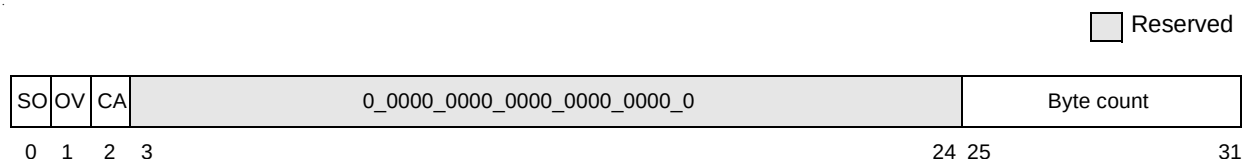
Figure D-6. XER Register
