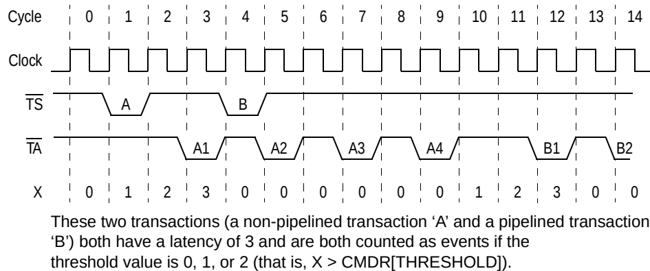
Figure 16-6. Command Type 0 Threshold Example
