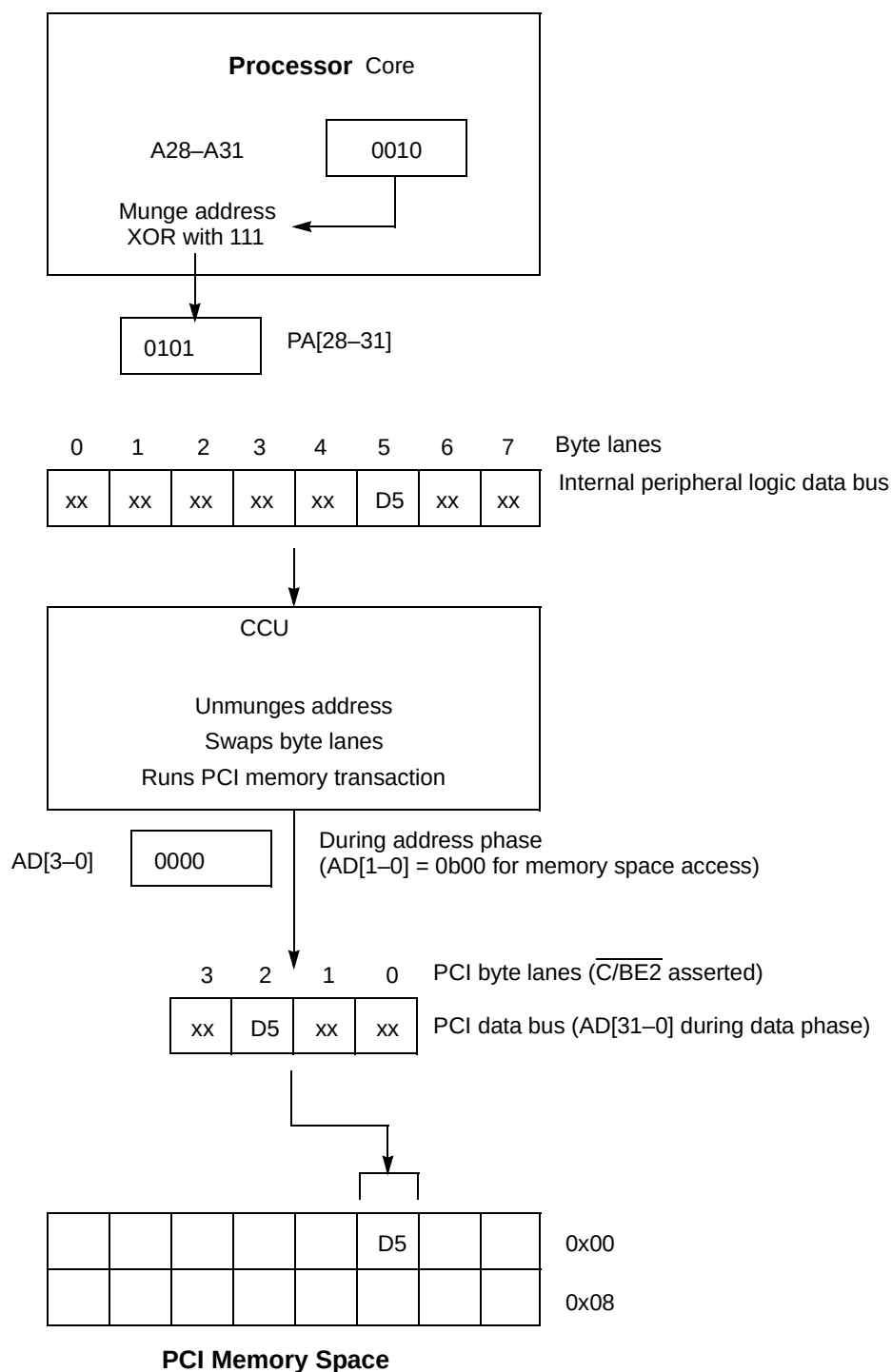
Figure A-6. One-Byte Transfer to PCI Memory Space—Little-Endian Mode
