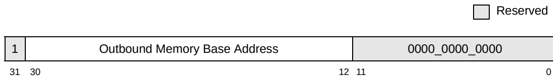
Figure 3-14. Outbound Memory Base Address Registers (OMBARN)— Offset 0x0_2300 and 0x0_2320
