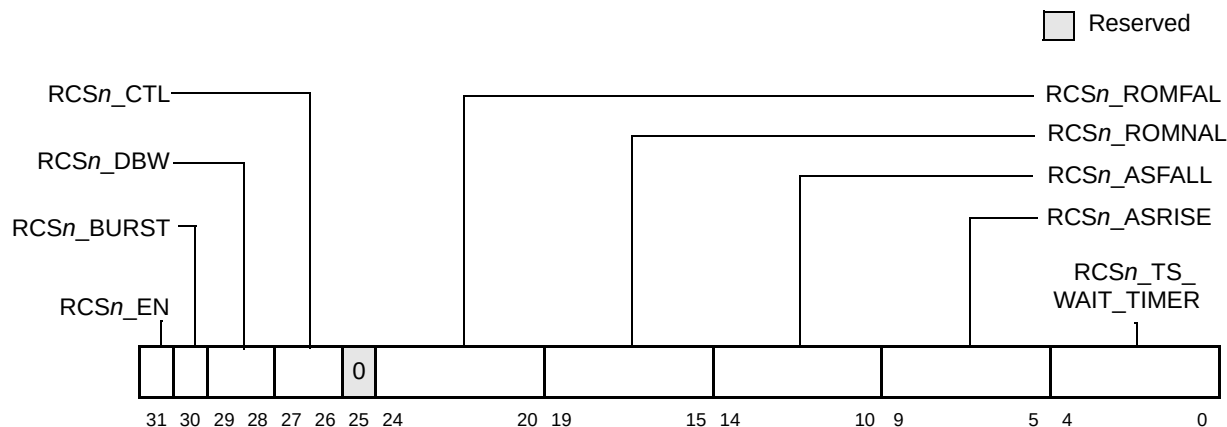
Figure 4-28. ERCCR1 and ERCCR2—0xD0, 0xD4
