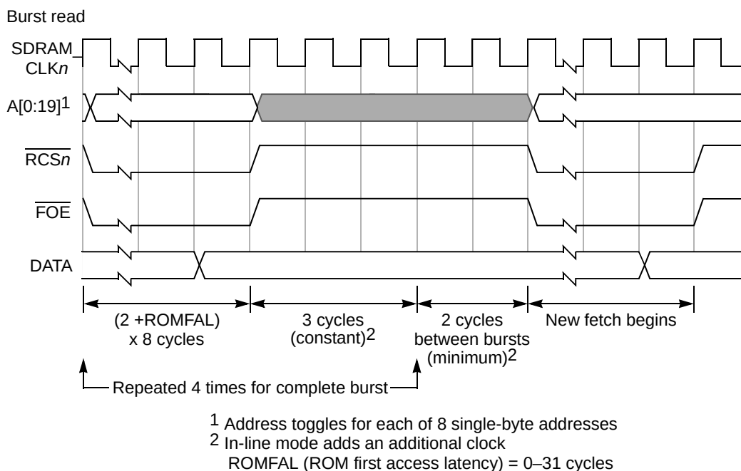
Figure 6-43. 8-Bit ROM/Flash Interface—Cache-Line Read Timing
