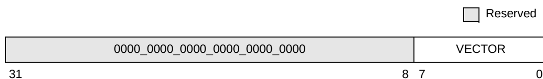
Figure 11-19. Processor Interrupt Acknowledge Register (IACK)
