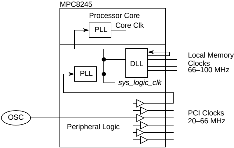
Figure 2-5. Clocking Solution—Small Load Requirements
