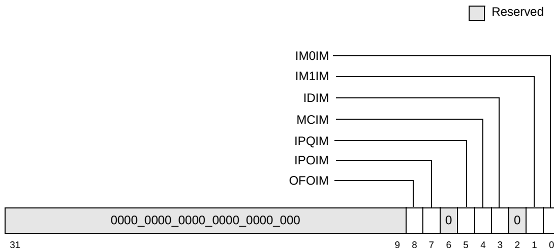
Figure 9-10. Inbound Message Interrupt Mask Register (IMIMR)
