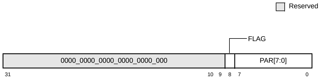
Figure 17-20. Parity Error Capture Monitor—Offsets 0xF_F014, 0xF14
