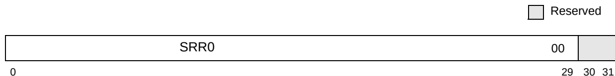
Figure D-18. Machine Status Save/Restore Register 0 (SRR0)
