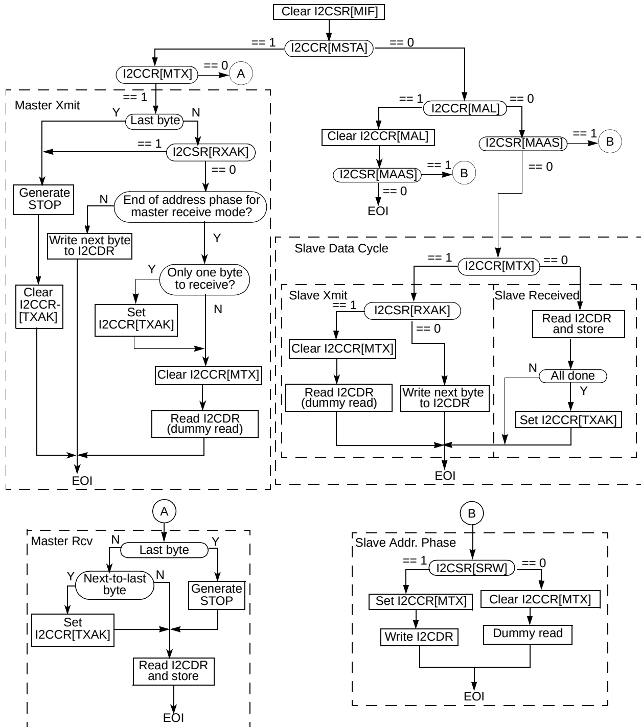
Figure 10-8. Example I²C Interrupt Service Routine Flowchart
