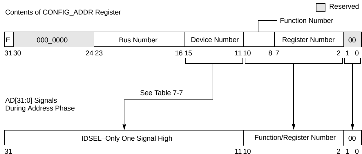
Figure 7-14. Type 0 Configuration Translation
