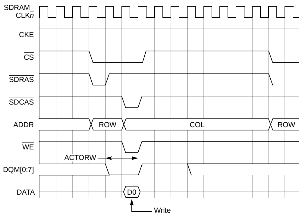
Figure 6-13. SDRAM Single-Beat Write Timing (SDRAM Burst Length = 4)
