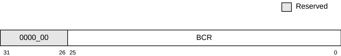
Figure 8-12. Byte Count Register (BCR)
