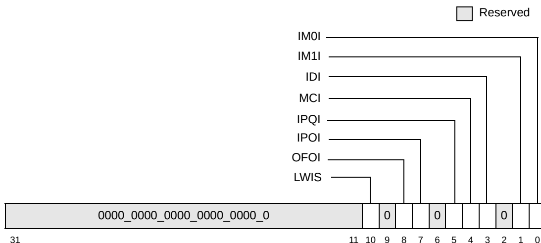
Figure 9-9. Inbound Message Interrupt Status Register (IMISR)
