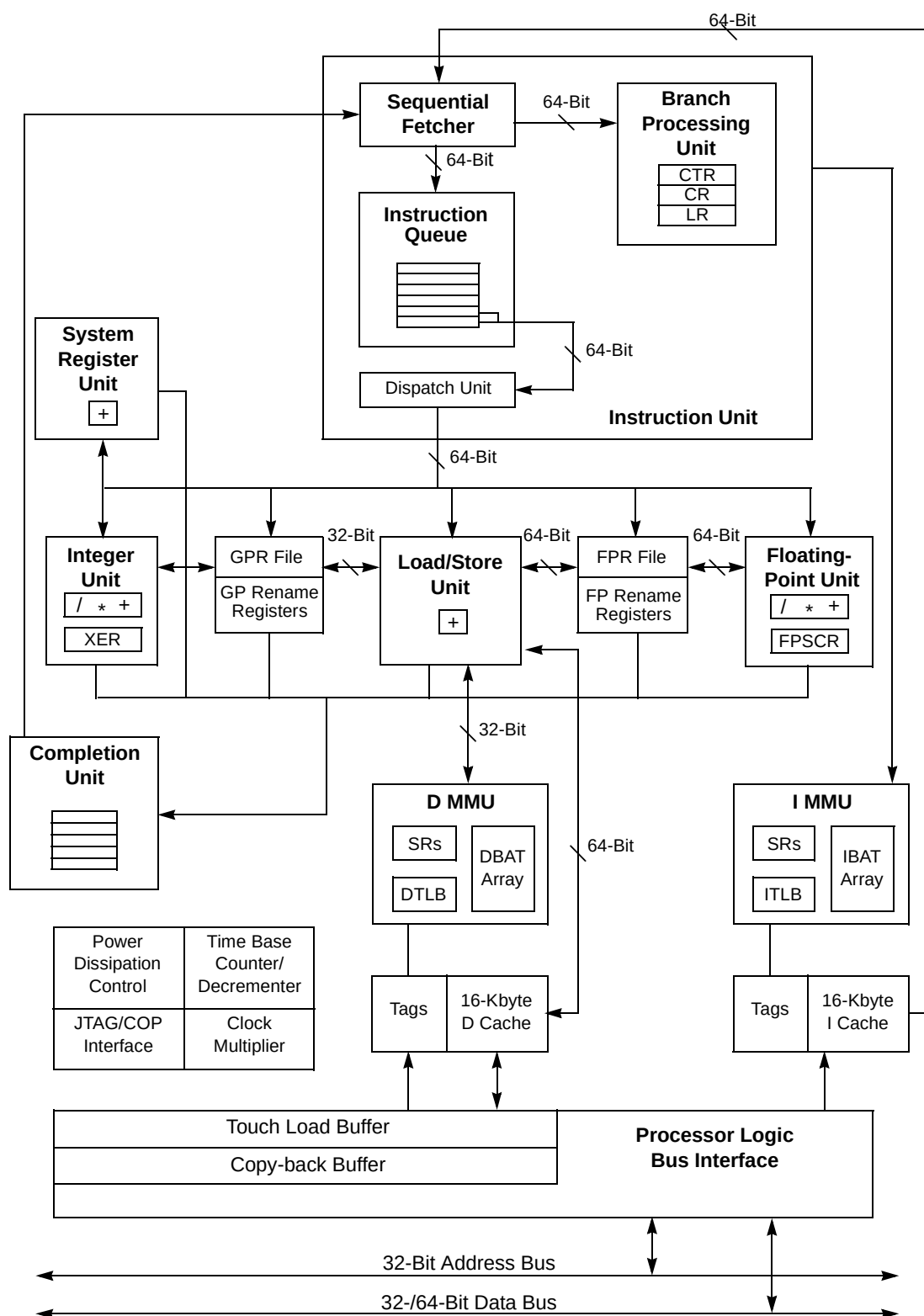
Figure 1-5. MPC8245 Integrated Processor Core Block Diagram
