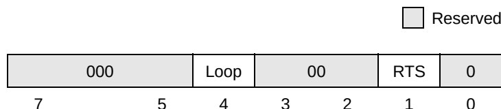
Figure 12-11. Modem Control Register (UMCR)
