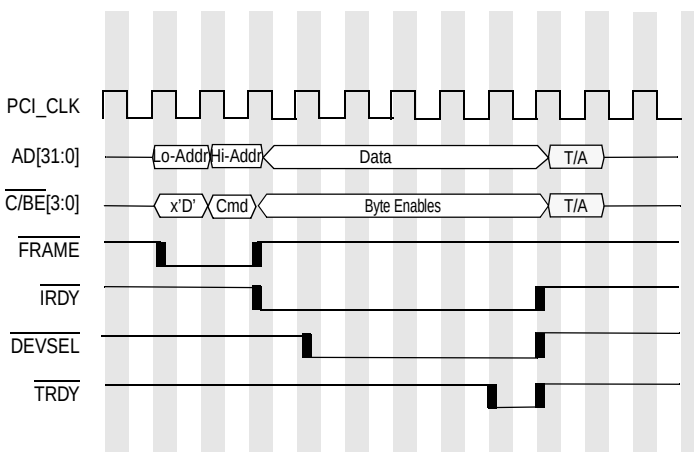
Figure 7-10. DAC Single-Beat Write Example
