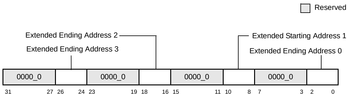
Figure 4-13. Extended Memory Ending Address Register 1—0x98
