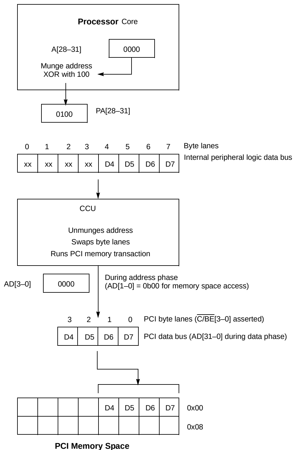
Figure A-8. Four-Byte Transfer to PCI Memory Space—Little-Endian Mode
