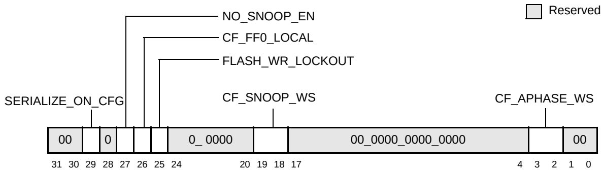
Figure 4-18. Processor Interface Configuration Register 2 (PICR2)—0xAC
