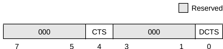
Figure 12-13. Modem Status Register (UMSR)
