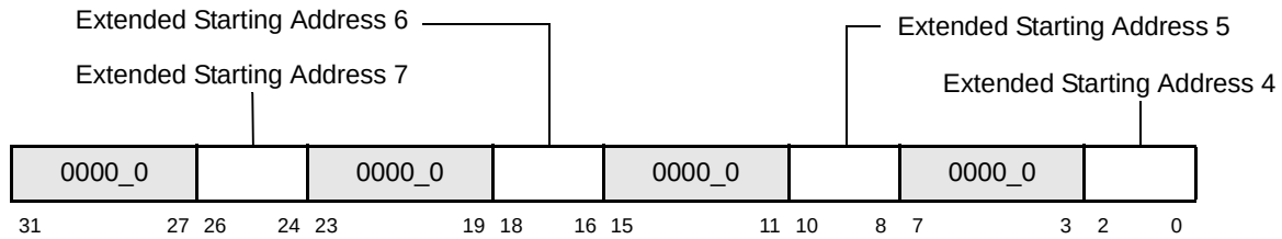
Figure 4-10. Extended Memory Starting Address Register 2—0x8C
