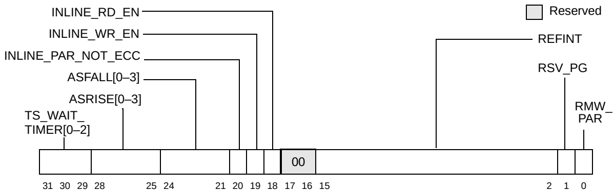
Figure 4-33. Memory Control Configuration Register 2 (MCCR2)—0xF4
