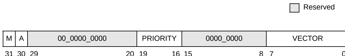
Figure 11-14. Global Timer Vector/Priority Registers (GTVPR)
