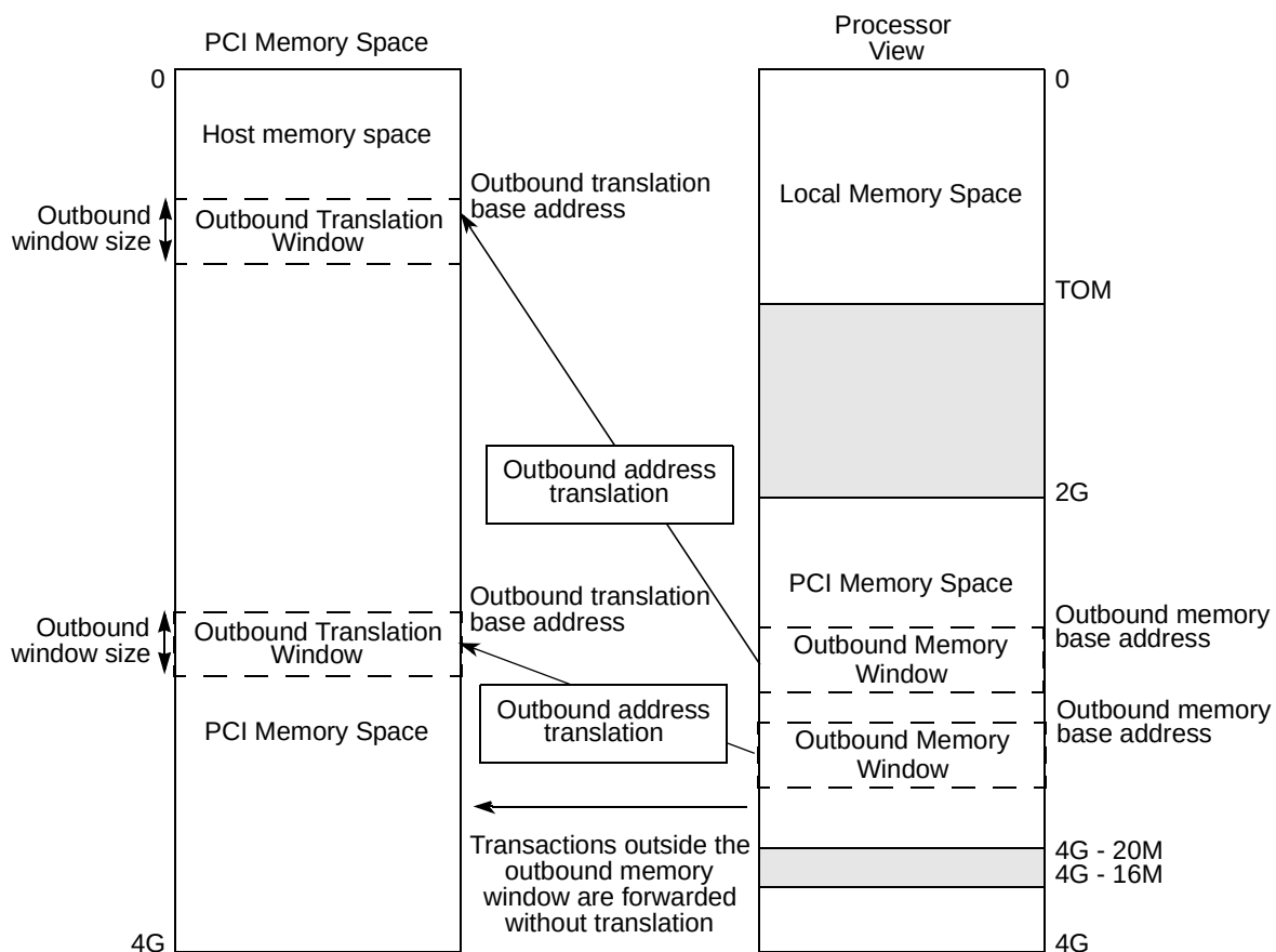
Figure 3-9. Outbound PCI Address Translation, OTHBAR = 0
