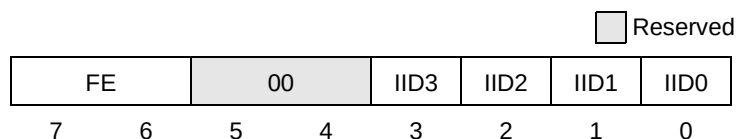
Figure 12-8. Interrupt ID Register (UIIR)
