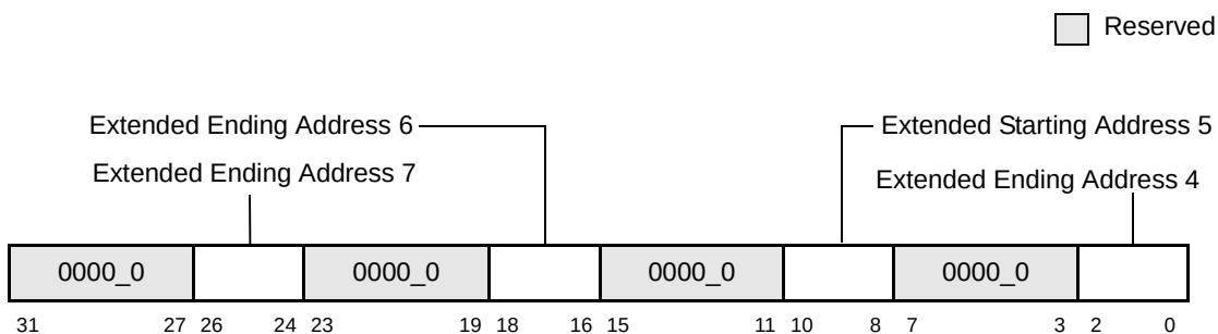
Figure 4-14. Extended Memory Ending Address Register 2—0x9C
