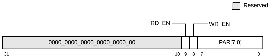
Figure 17-17. Parity Error Injection Mask—Offsets 0xF_F008, 0xF08
