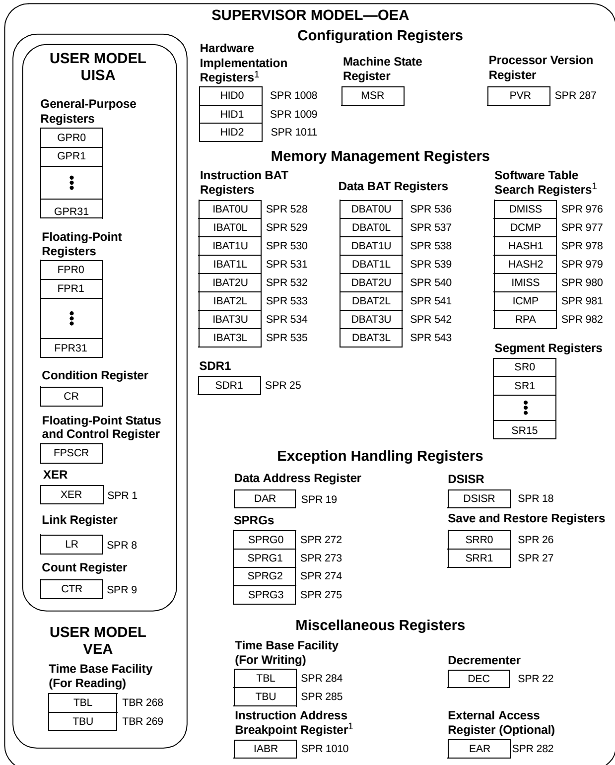
Figure 5-2. MPC8245 Programming Model—Registers
