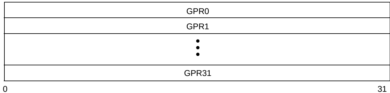
Figure D-2. General-Purpose Registers (GPRs)
