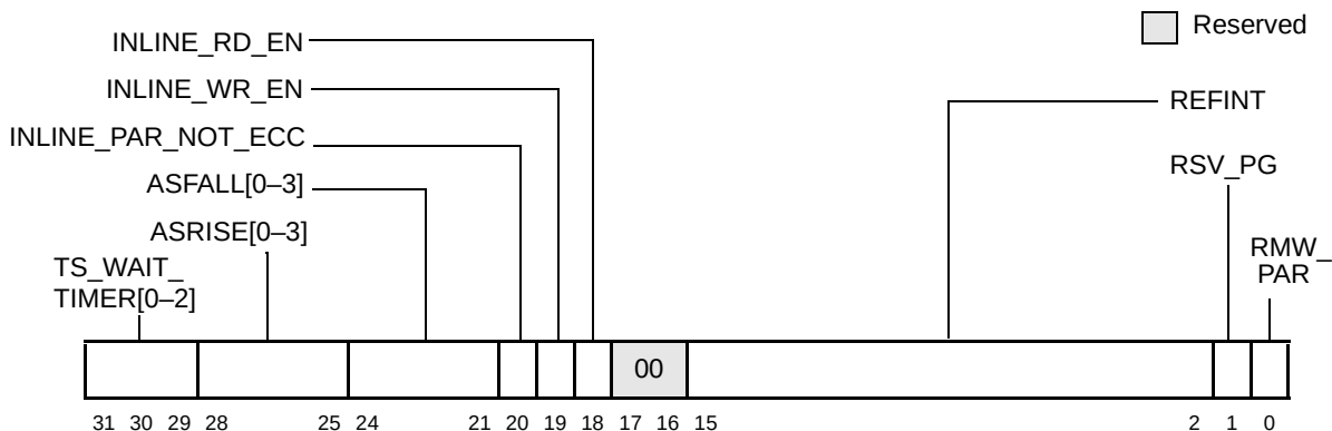
Figure 4-34. Memory Control Configuration Register 2 (MCCR2)—0xF4
