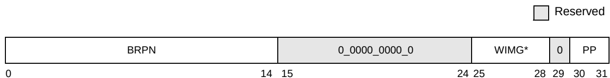
Figure D-13. Lower BAT Register
