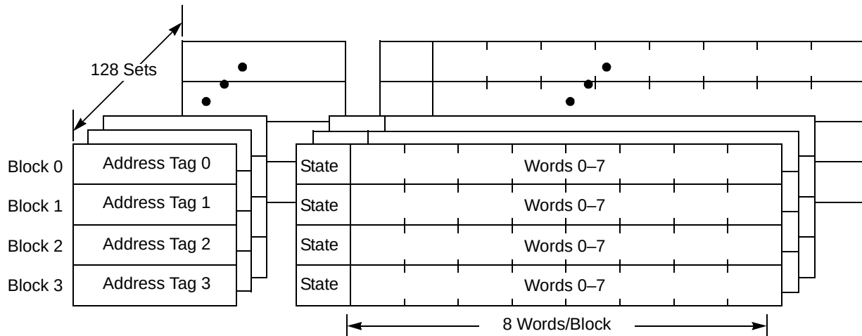
Figure 5-6. Data Cache Organization
