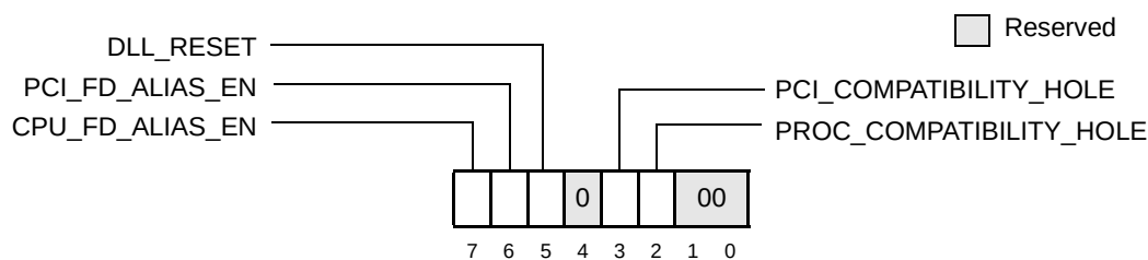
Figure 4-30. Address Map B Options Register (AMBOR)—0xE0
