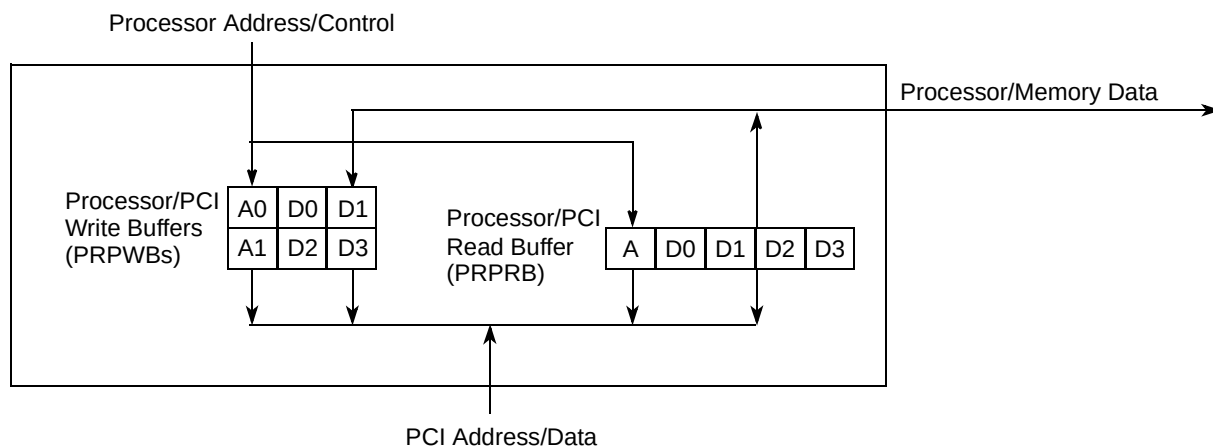
Figure 13-3. Processor/PCI Buffers
