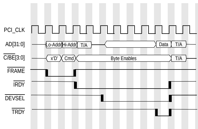
Figure 7-8. DAC Single-Beat Read Example
