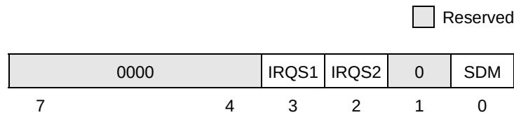
Figure 12-17. DUART Configuration Register (DCR)
