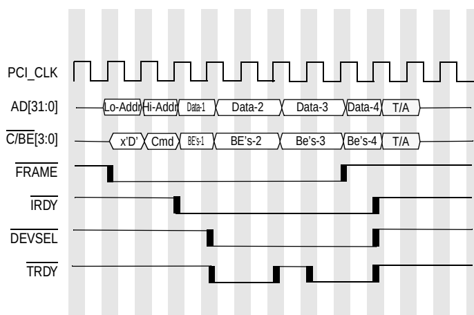
Figure 7-11. DAC Burst Write Example
