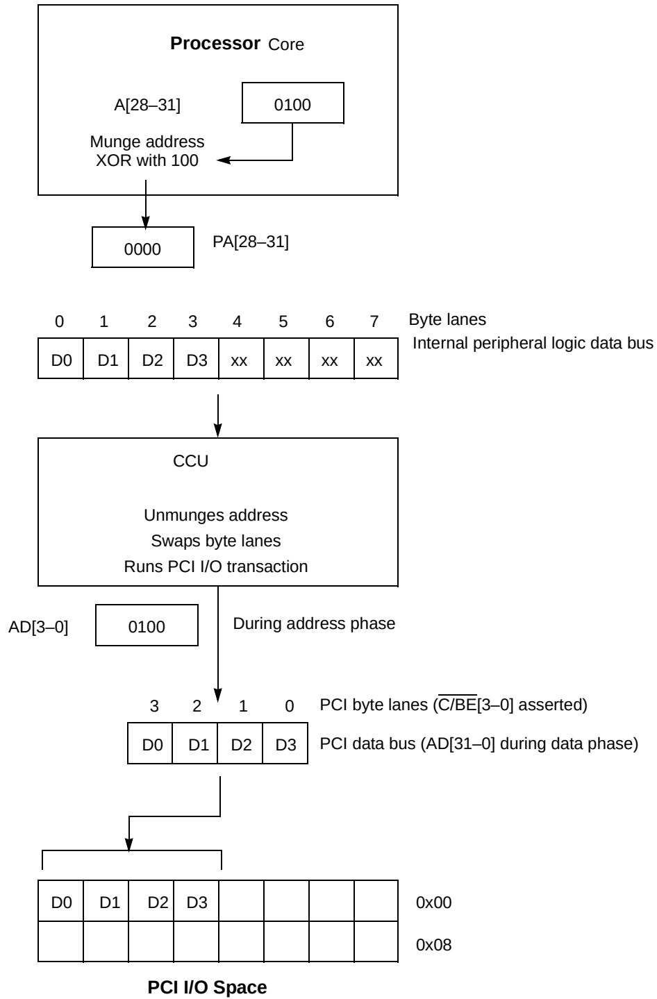
Figure A-11. Four-Byte Transfer to PCI I/O Space—Little-Endian Mode
