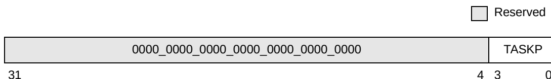
Figure 11-18. Processor Current Task Priority Register (PCTPR)
