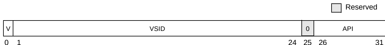
Figure D-23. DCMP and ICMP Registers
