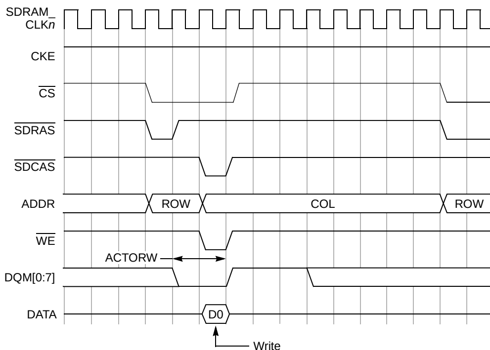
Figure 6-10. SDRAM Single-Beat Write Timing (SDRAM Burst Length = 4)
