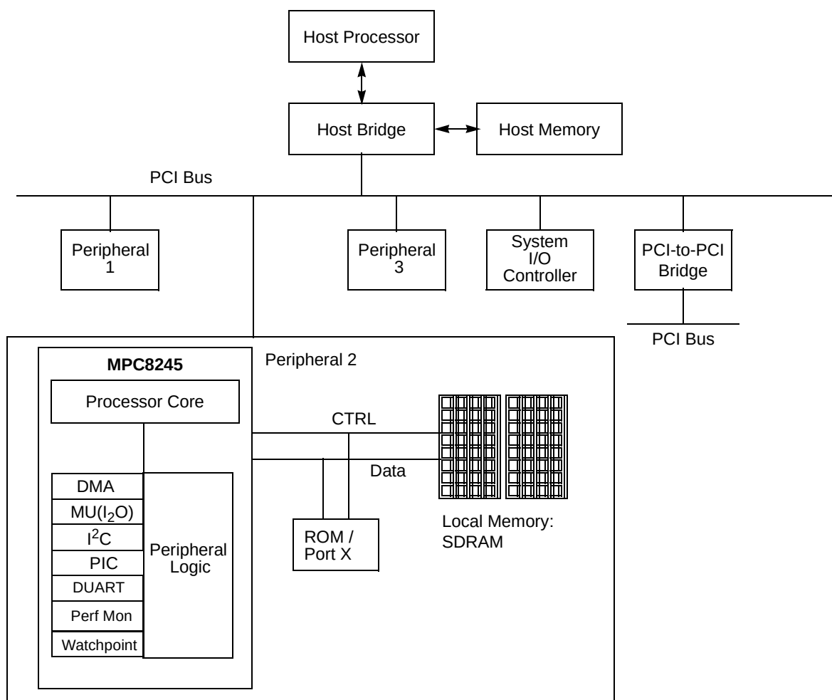
Figure 1-3. Embedded System Using an MPC8245 as a Peripheral Processor
