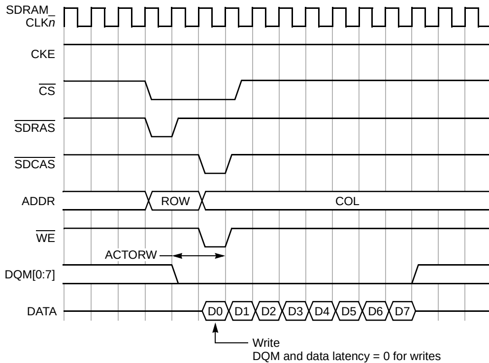
Figure 6-12. SDRAM Eight-Beat Burst Write Timing—32-Bit Mode
