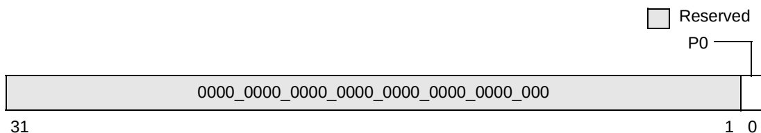
Figure 11-15. Global Timer Destination Register (GTDR)
