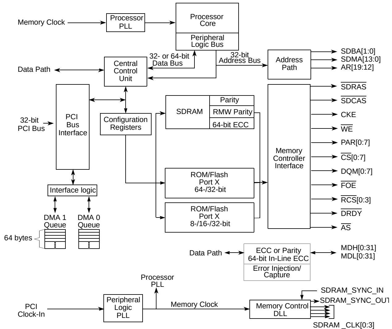
Figure 6-1. Block Diagram for Memory Interface
