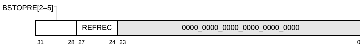
Figure 4-35. Memory Control Configuration Register 3 (MCCR3)—0xF8
