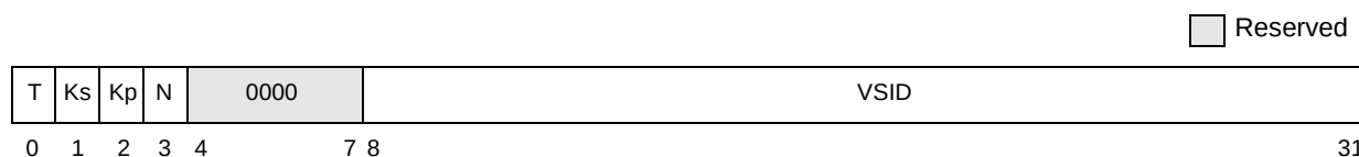
Figure D-15. Segment Register Format (T = 0)
