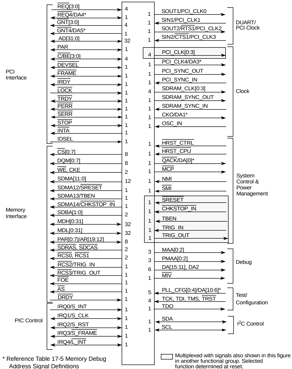
Figure 2-1. MPC8245 Signal Groups
