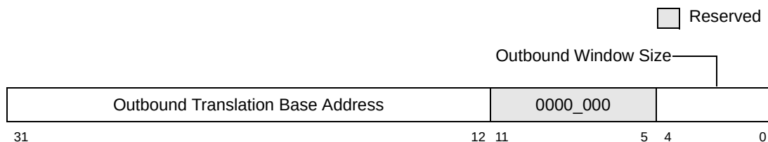
Figure 3-15. Outbound Translation Window Registers (OTWRn)— Offset 0x0_2308 and 0x0_2328
