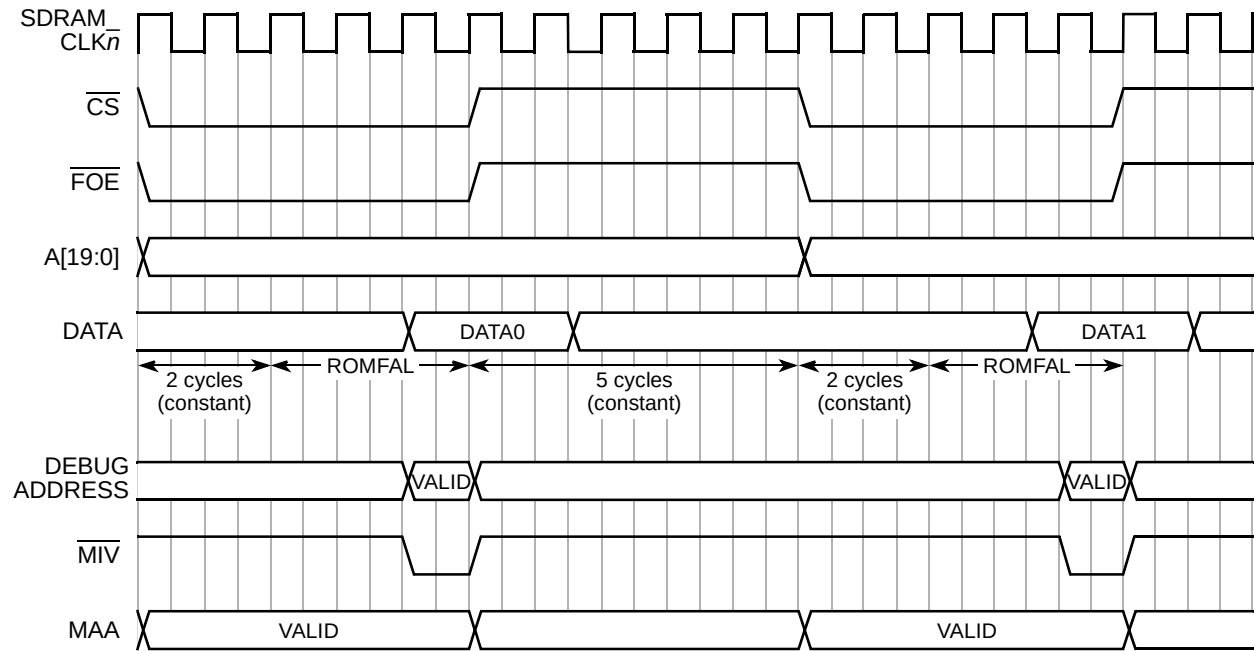
Figure 17-12. Example Flash Debug Address, \overline{\text{MIV}} , and MAA Timings For Single-Byte Read
