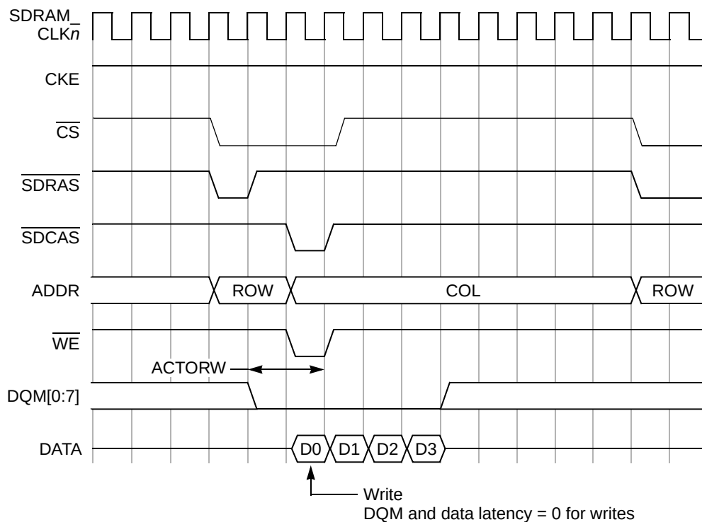
Figure 6-11. SDRAM Four-Beat Burst Write Timing—64-Bit Mode
