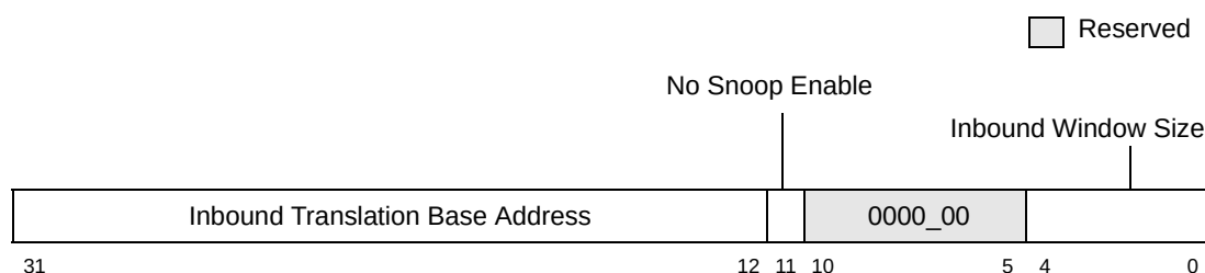
Figure 3-12. Inbound Translation Window Register (ITWR n )—Offset 0x0_2310 and 0x0_2330
