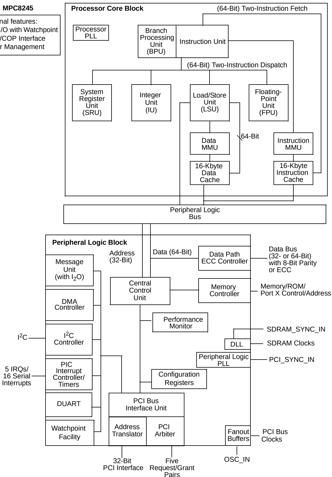
Figure 1-1. MPC8245 Integrated Processor Functional Block Diagram
