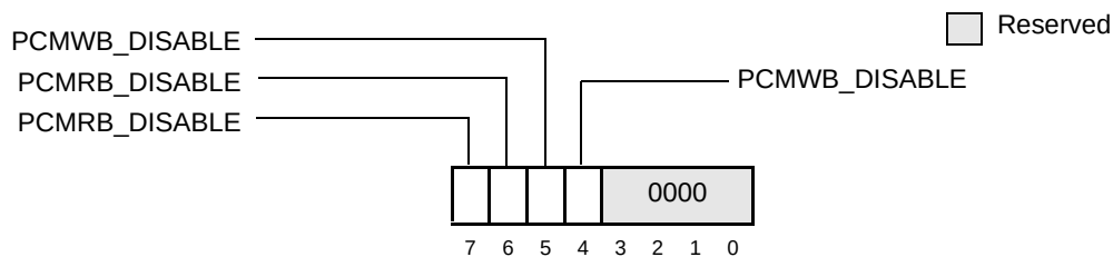
Figure 4-31. PCI/Memory Buffer Configuration Register (PCMBCCR)—0xE1
