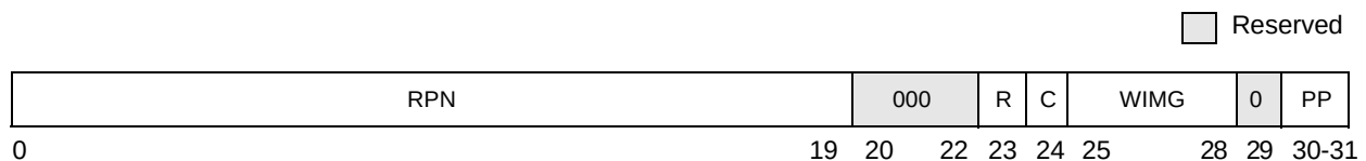
Figure D-25. Required Physical Address Register (RPA)
