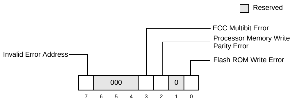
Figure 4-25. Error Detection Register 2 (ErrDR2)—0xC5
