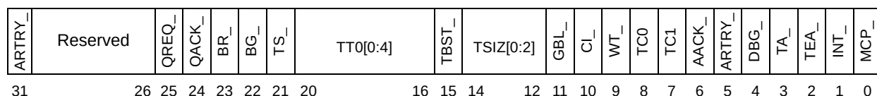
Figure 18-3. Watchpoint #2 Control Trigger Register (WP2_CNTL_TRIG)— Offsets 0xF_F030, 0xF30
