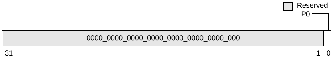
Figure 11-8. Processor Initialization Register (PI)
