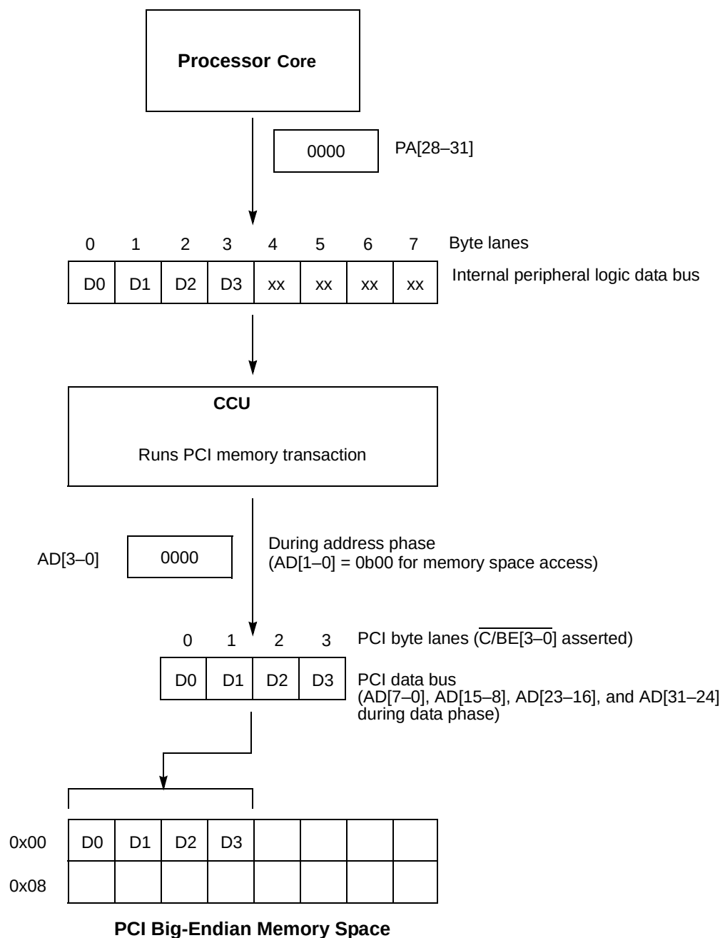
Figure A-1. Four-Byte Transfer to PCI Memory Space—Big-Endian Mode
