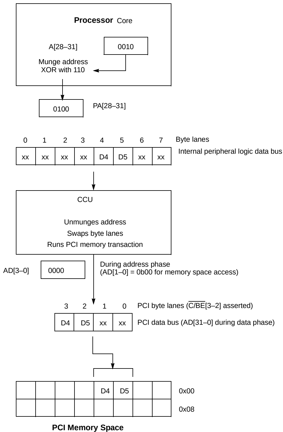
Figure A-7. Two-Byte Transfer to PCI Memory Space—Little-Endian Mode
