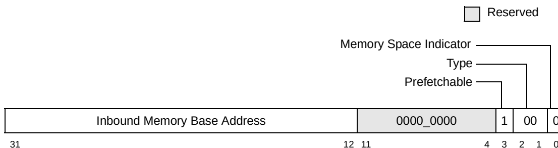
Figure 3-11. Local Memory Base Address Registers (LMBAR n )—Offset 0x10 and 0x18
