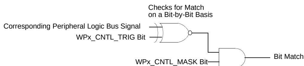
Figure 18-6. Bit Match Generation for Watchpoint Trigger Bit Settings
