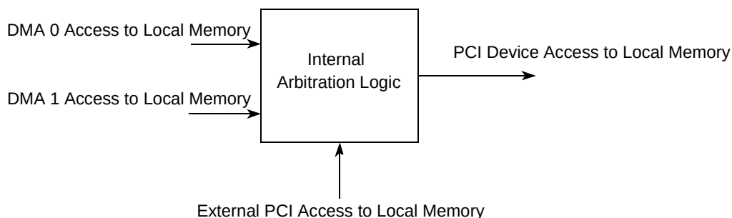
Figure 13-5. PCI/DMA Arbitration for Local Memory Accesses
