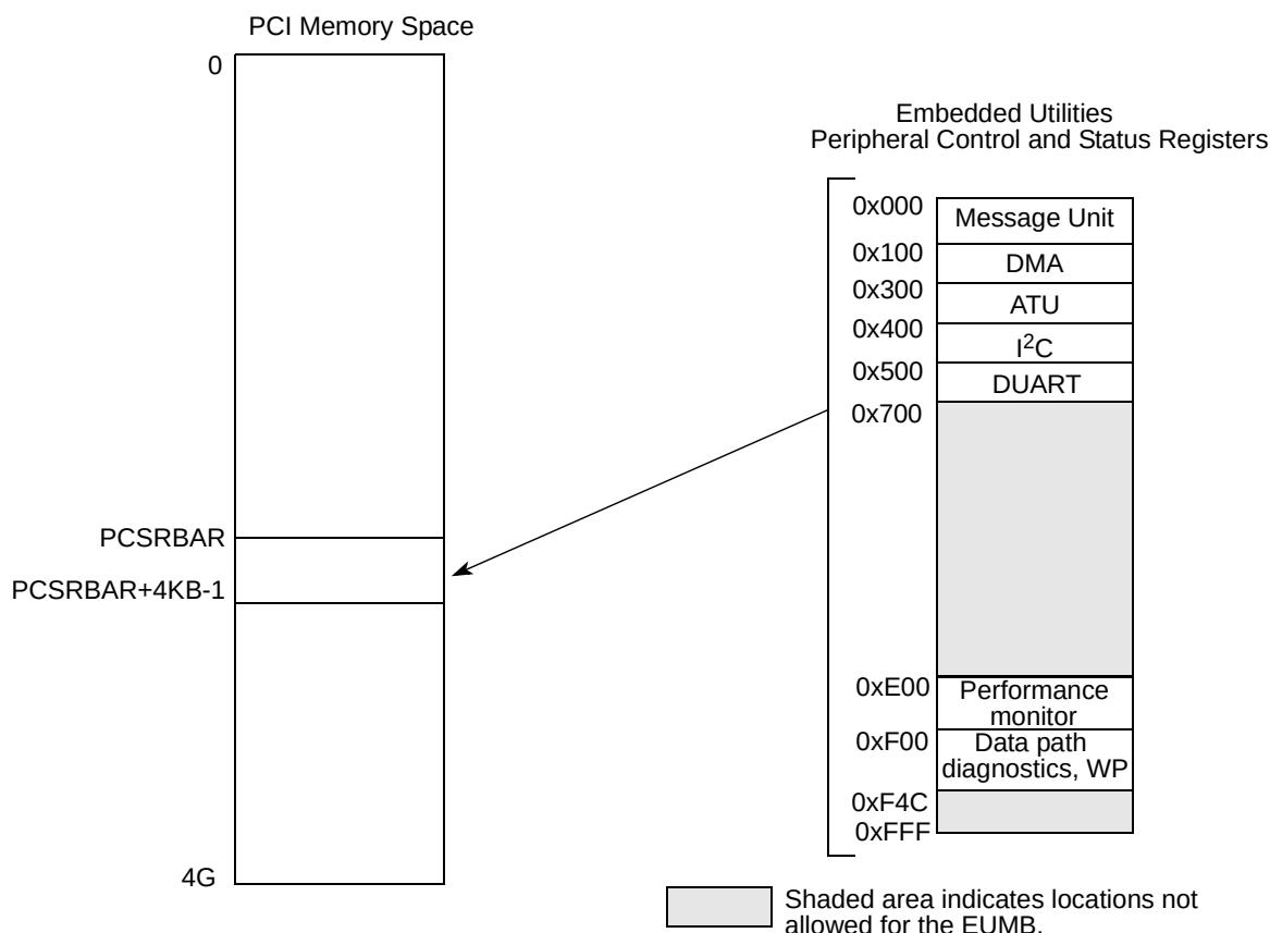
Figure 3-17. Embedded Utilities Memory Block Mapping to PCI Memory
