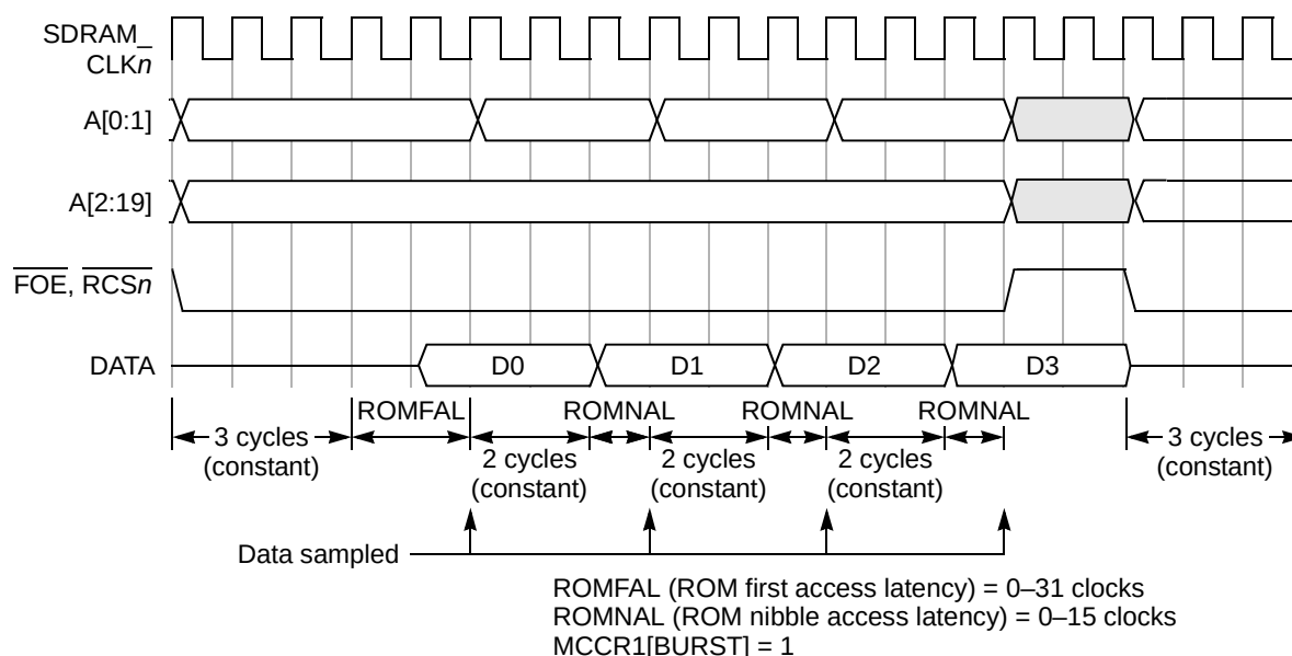
Figure 6-39. Read Access Timing (Cache Block) for Burst ROM/Flash Devices—64-Bit (Wide) Data Path
