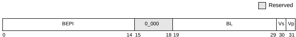
Figure D-12. Upper BAT Register
