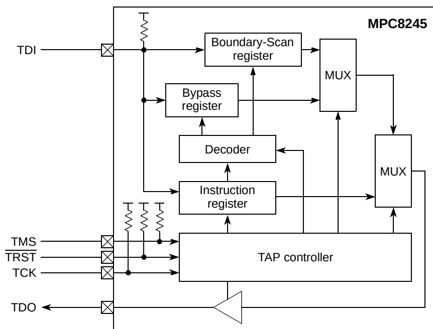
Figure 17-21. JTAG Interface Block Diagram
