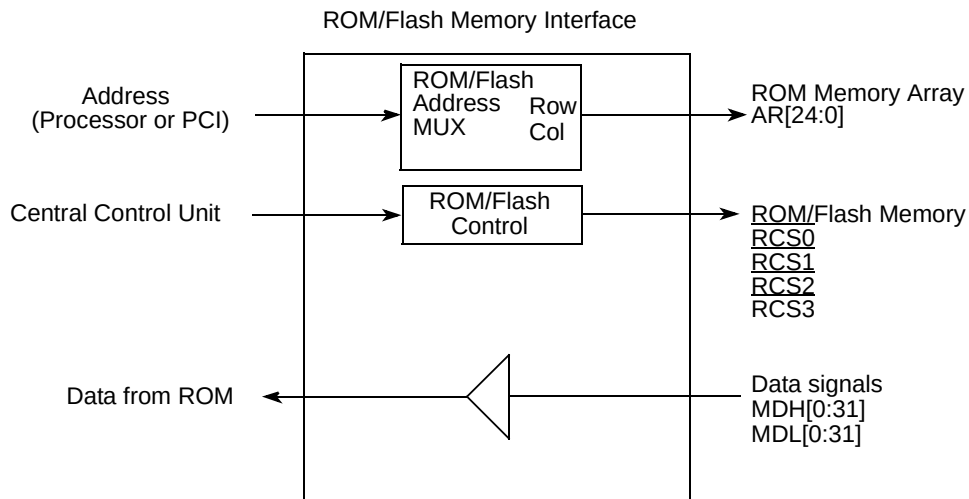
Figure 6-28. ROM Memory Interface Block Diagram
