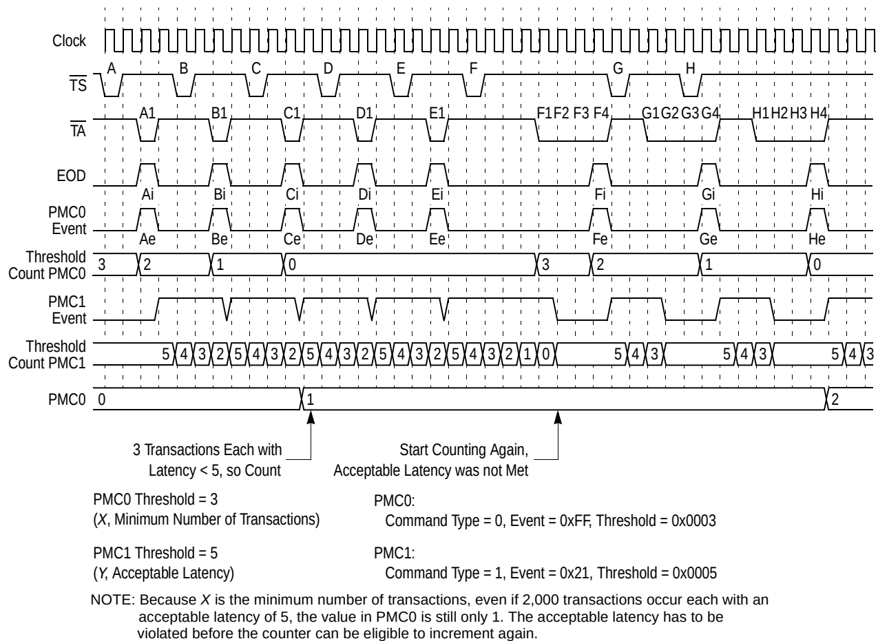
Figure 16-7. Processor Burstiness Example
