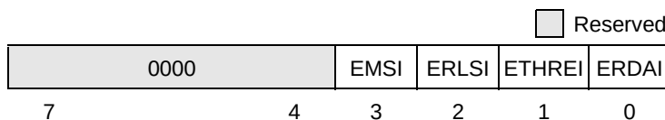
Figure 12-7. Interrupt Enable Register (UIER)
