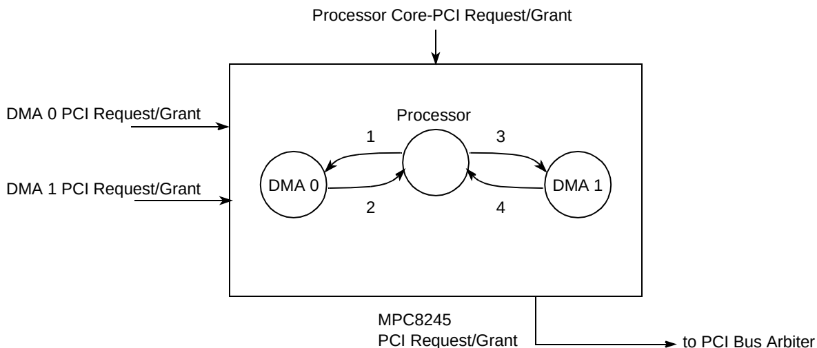
Figure 7-1. Internal Processor DMA Arbitration for PCI Bus
