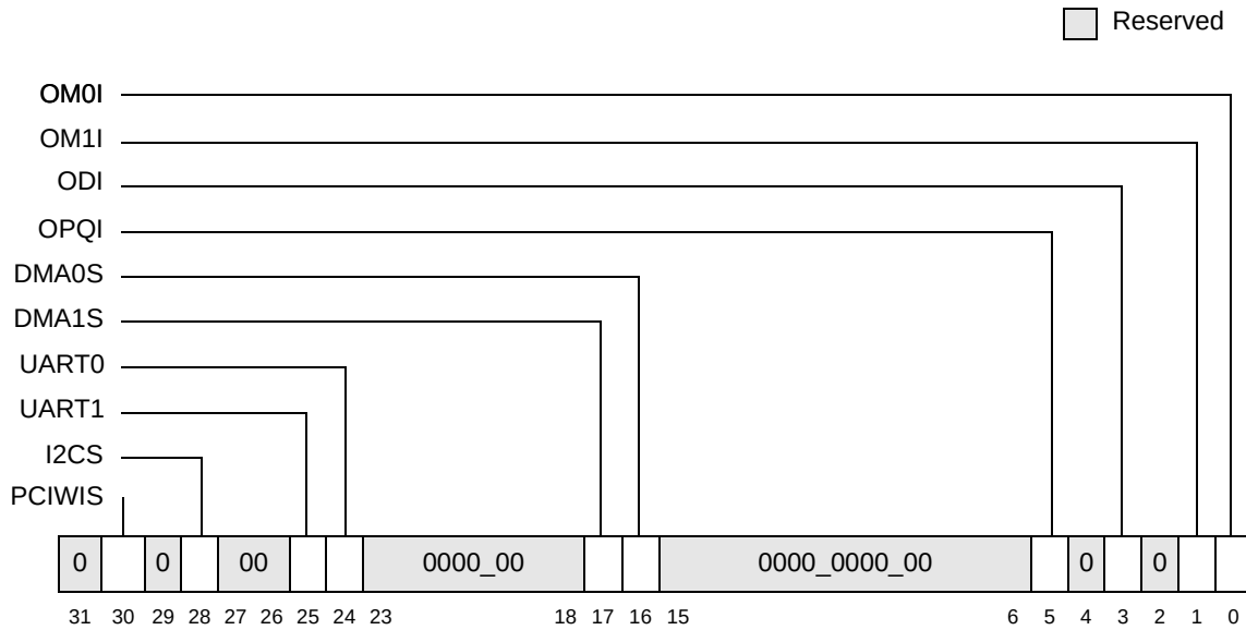
Figure 9-5. Outbound Message Interrupt Status Register (OMISR)
