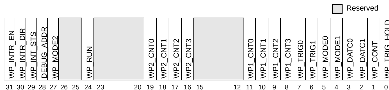
Figure 18-11. Watchpoint Control Register (WP_CONTROL)— Offsets 0xF_F048, 0xF48
