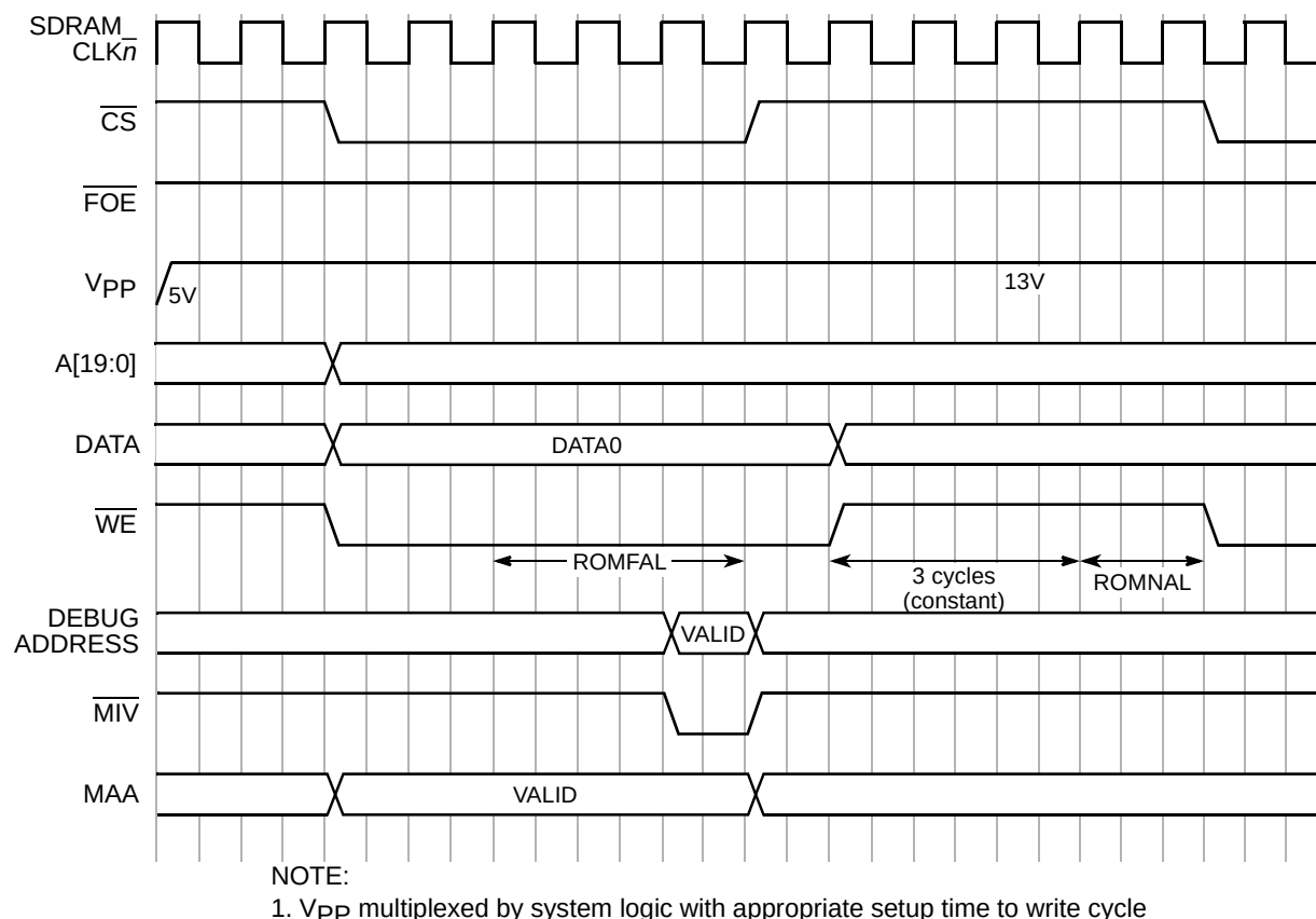
Figure 17-13. Example Flash Debug Address, \overline{MIV} , and MAA Timings for Write Operation
