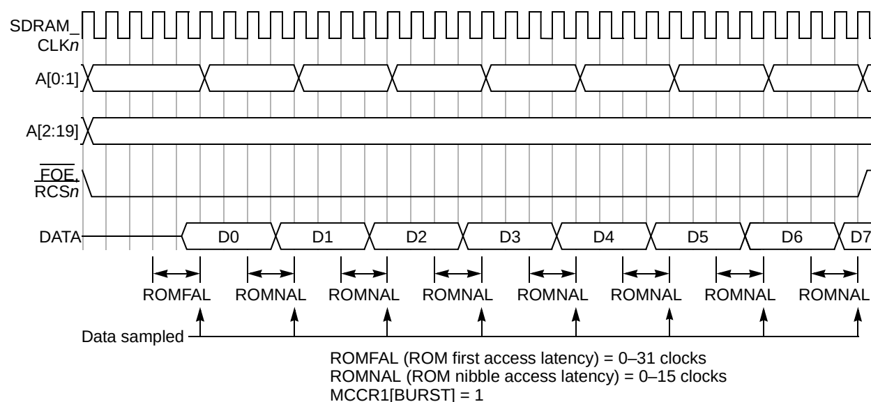
Figure 6-40. Read Access Timing (Cache Block) for Burst ROM/Flash Devices—32-Bit (Wide) Data Path
