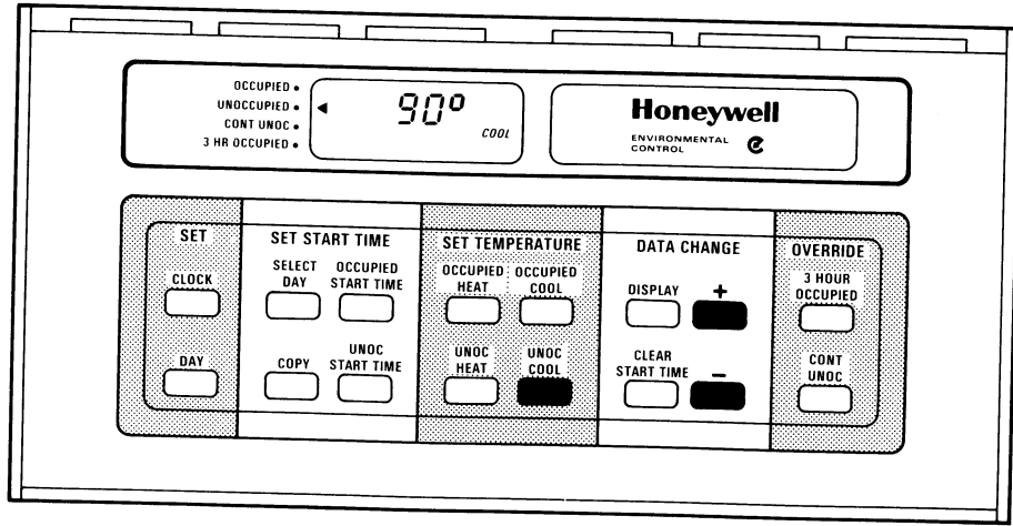
KEYS USED FOR SETTING THE UNOCCUPIED COOL SETPOINT
