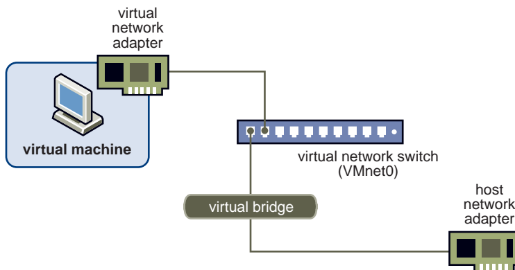
Figure 14-1. Bridged Networking Setup
