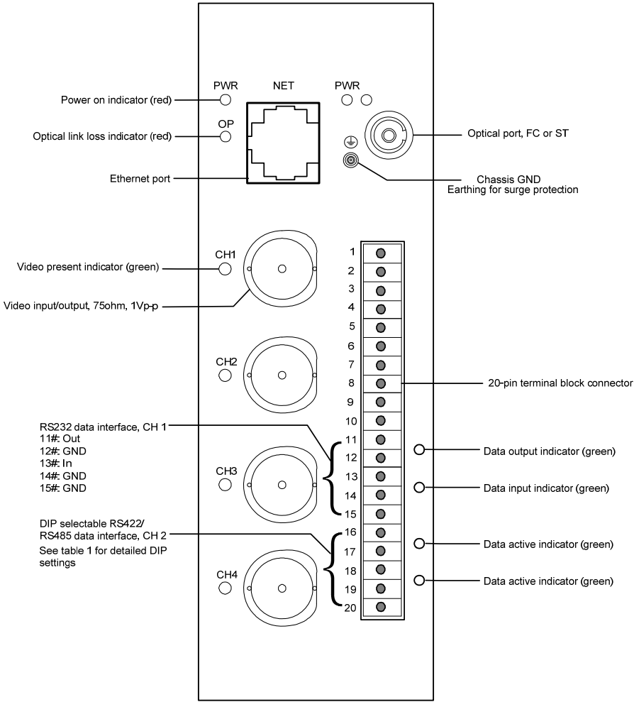
Figure 4. N3754T/R-1D1B-IP & N3554T/R-1D1B-IP
