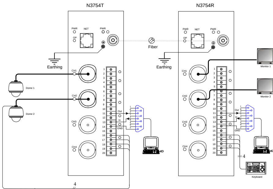
Figure 11. Four video channels with one RS232, one DIP selectable data and one Ethernet signal
