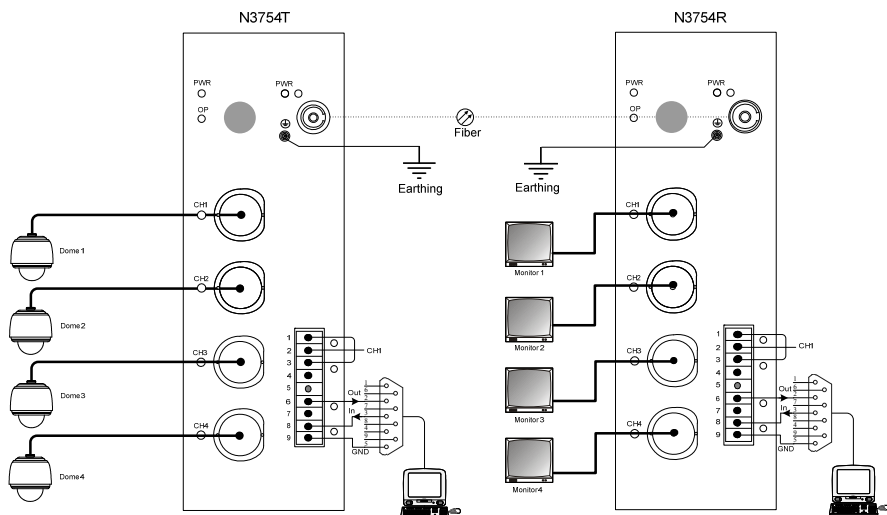
Four video channels with two RS232 data
