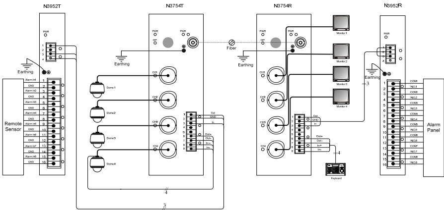
Figure 15. Contact closure signal connection
