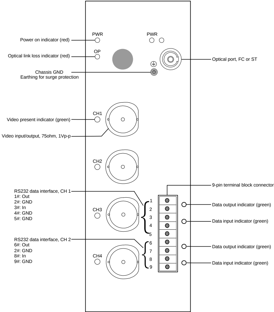
Figure 3. N3754T/R-2B & N3554T/R-2B
