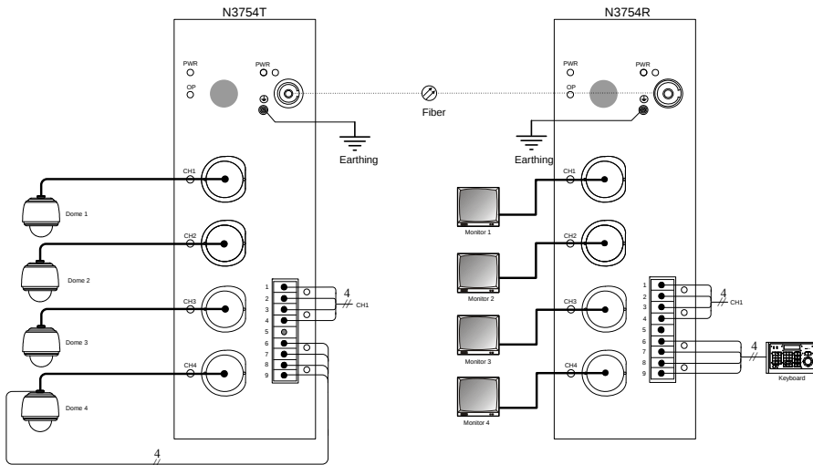
Figure 9. Four video channels with two DIP selectable data
