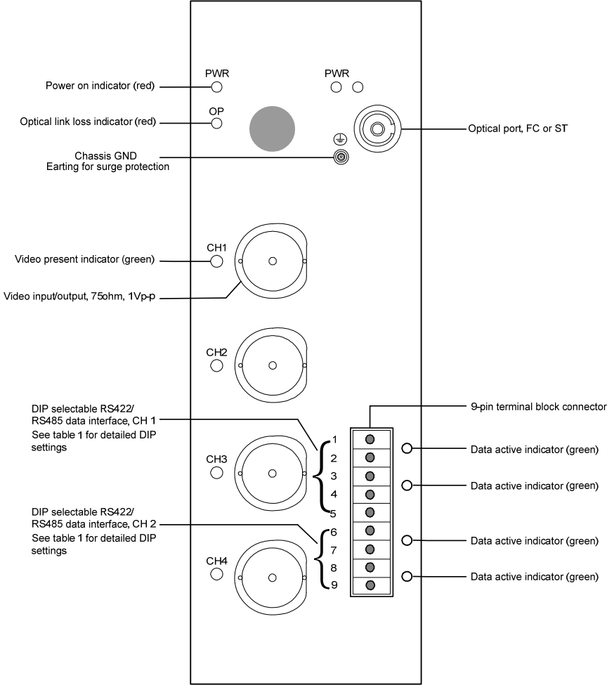
Figure 2. N3754T/R-2D & N3554T/R-2D
