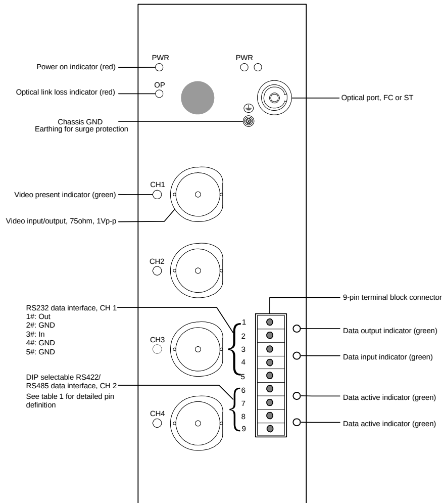
Figure 1. N3754T/R-1D1B & N3554T/R-1D1B
