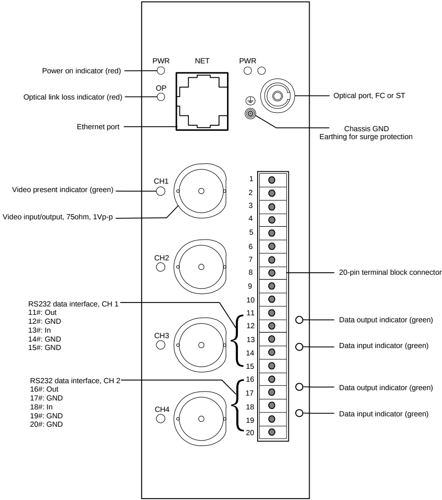
Figure 6. N3754T/R-2B-IP & N3554T/R-2B-IP
