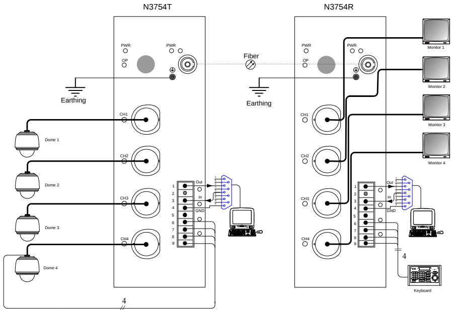
Figure 8. Four video channels with one RS232 and one DIP selectable data
