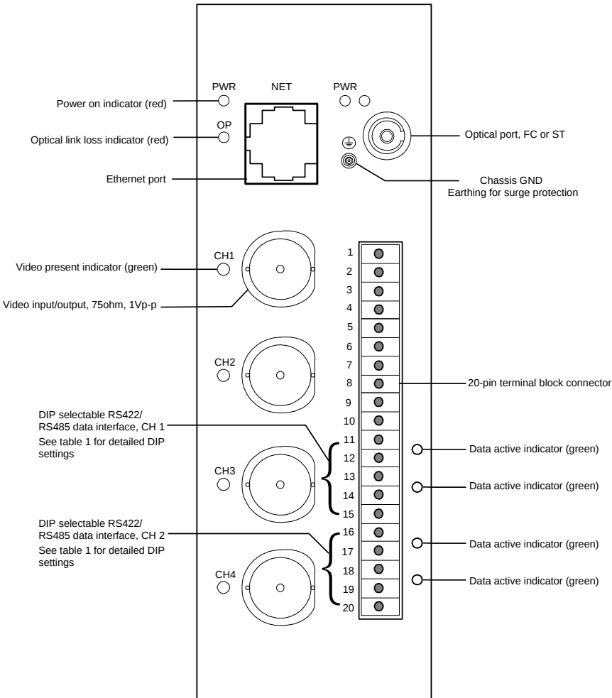
Figure 5. N3754T/R-2D-IP & N3554T/R-2D-IP
