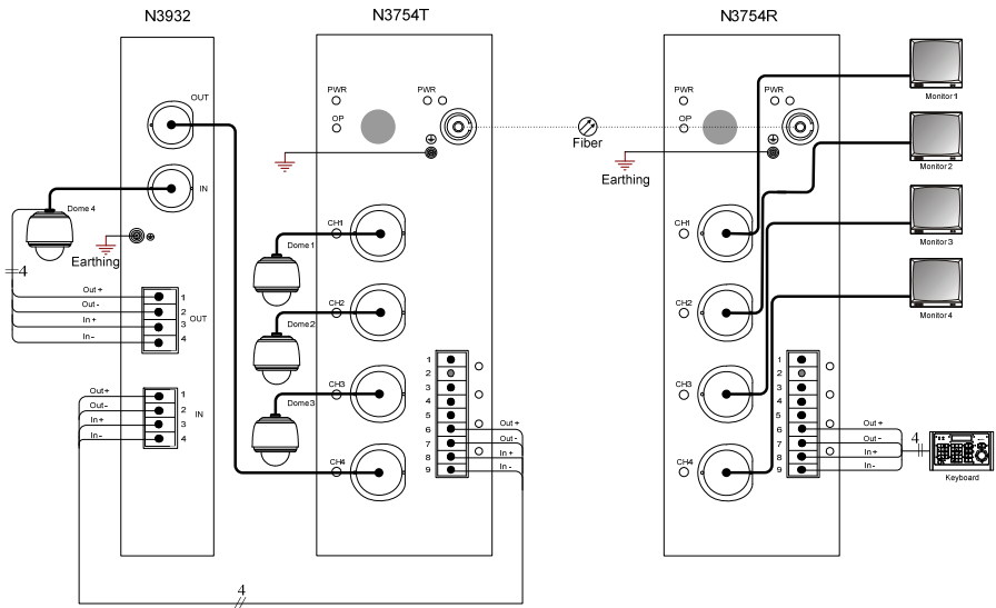
Figure 13. Lightning surge protection
