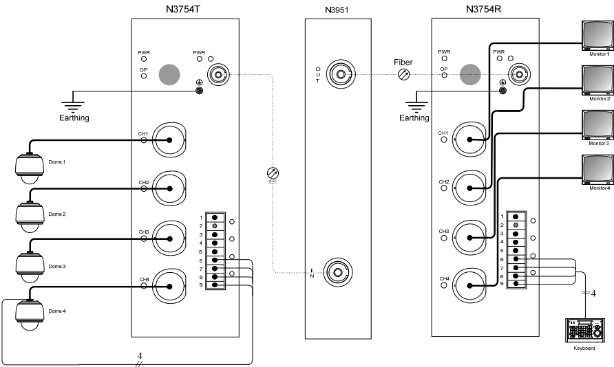
Figure 14. Transmission repeater
