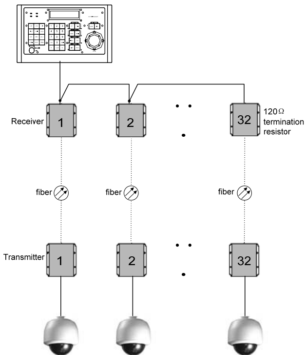
Figure 12. Daisy chain diagram
