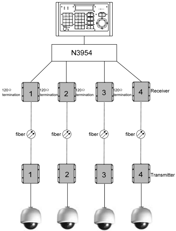
Figure 16. Code distributor diagram
