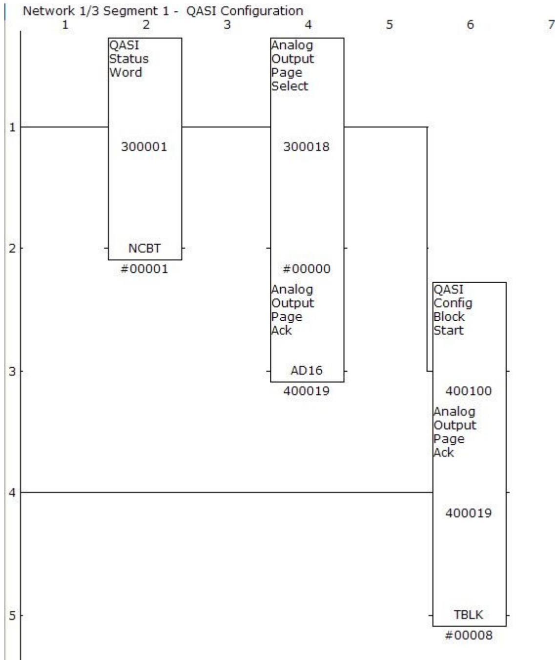
Figure 3.5: Configuration Block Network
