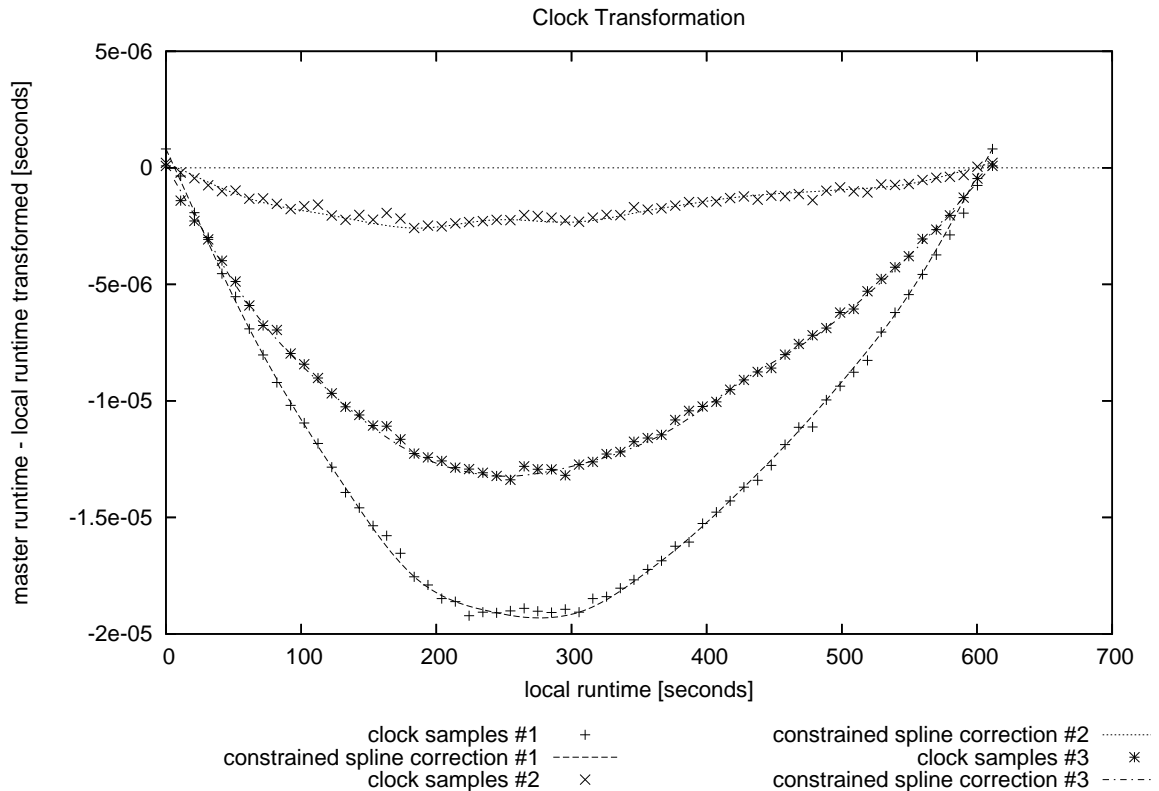
Figure 5.4: gettimeofday() without NTP.
