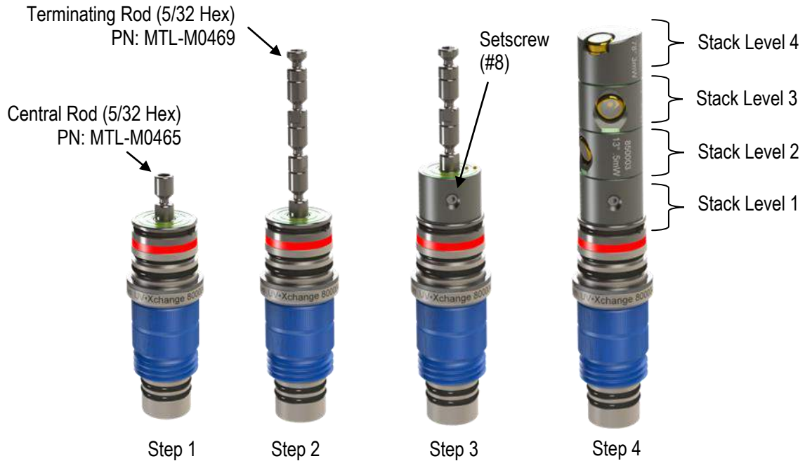
UV•Xchange module assembly procedure.
