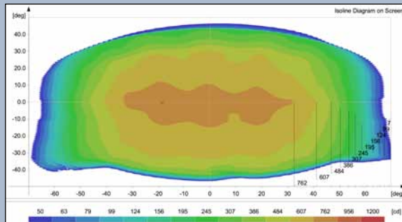
Halogen Light Source IsoCandela Plot (Luminous Intensity)
