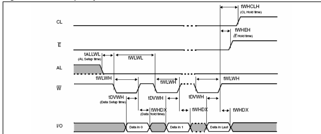
Figure 5. Data input cycle
