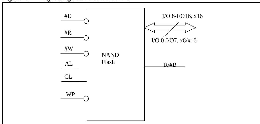
Figure 1. Logic diagram of NAND Flash
