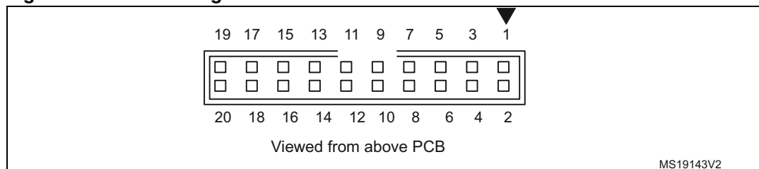
Figure 12. JTAG debug connector CN14
