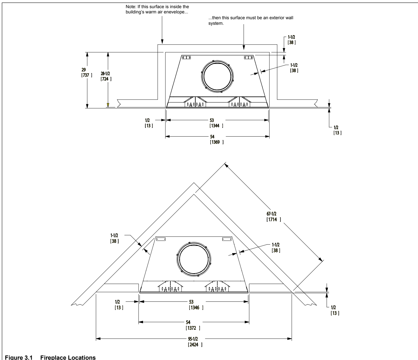
Figure 3.1 Fireplace Locations
