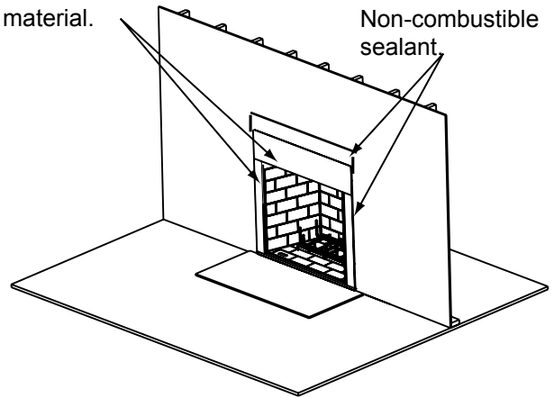
Figure 9.1 Non-combustible Facing
